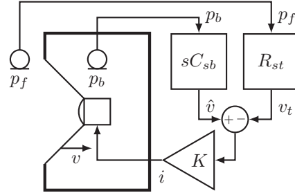
Figure 1. Control architecture
