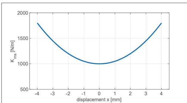
Figure 2. Simulated K_{ms}(x) .
