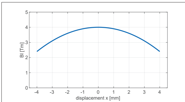
Figure 1. Simulated Bl(x) .
