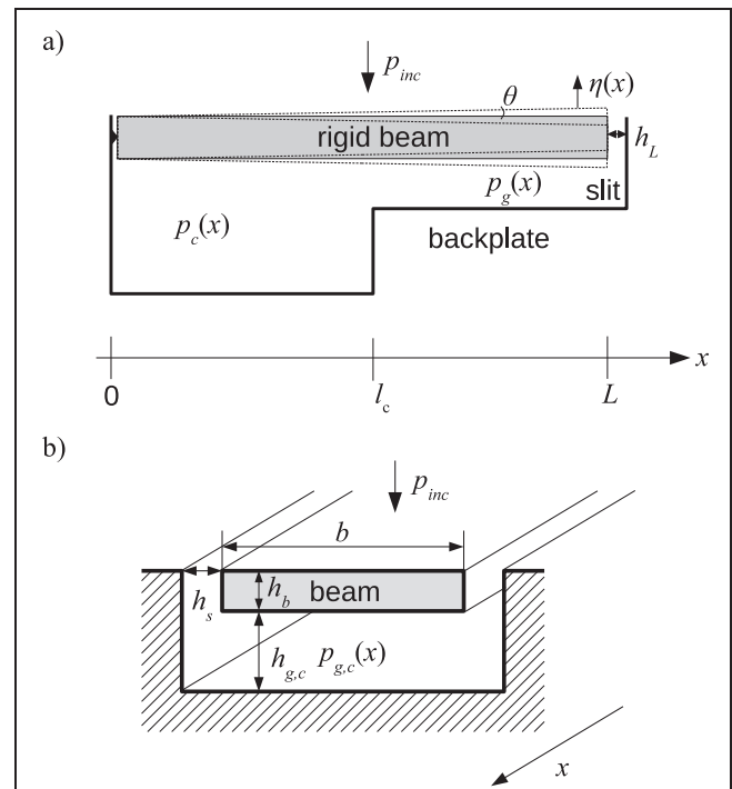
Figure 1. Geometry of the system: a) side view, b) cross-sectional view.
