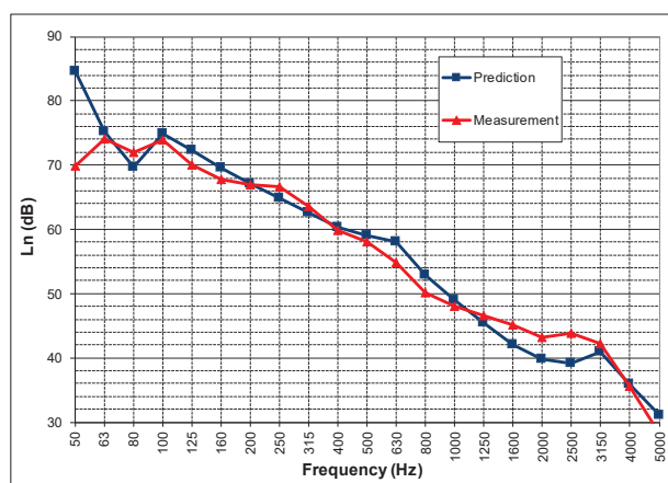
Figure 9. Comparison between predicted and measured impact sound level spectra – Basic floor.
