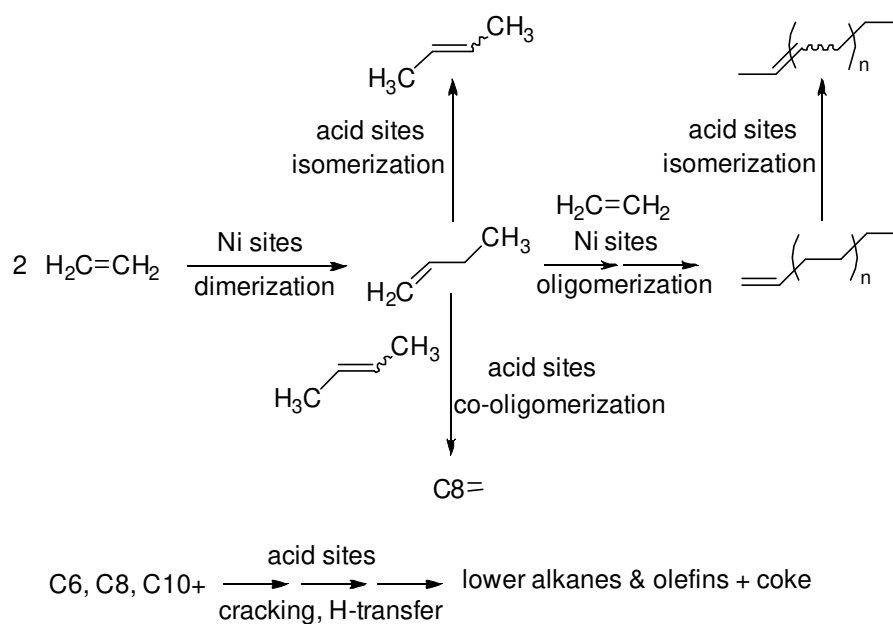
Scheme 1. Simplified scheme of the main reactions involved in ethylene oligomerization.
