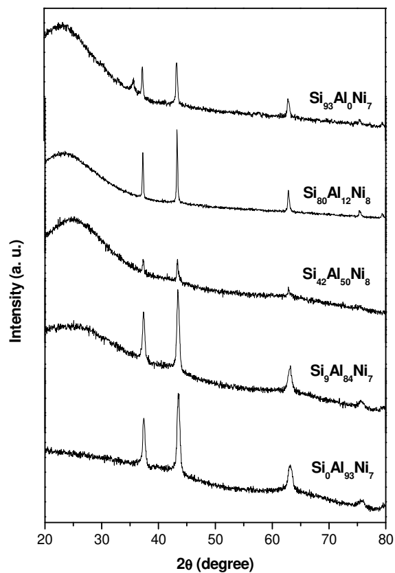
Figure 3: Powder XRD patterns of \text{Si}_x\text{Al}_y\text{Ni}_z samples.
