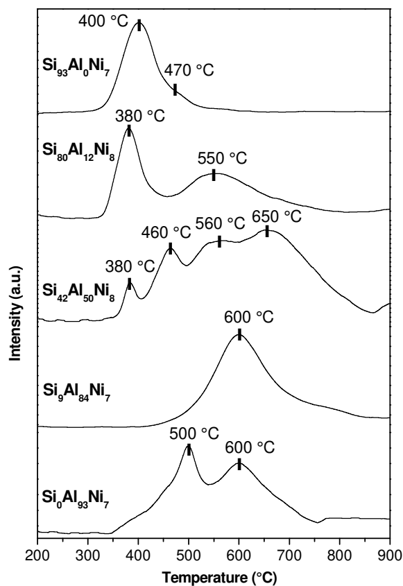
Figure 7: H 2 -TPR profiles of Si x Al y Ni z samples.
