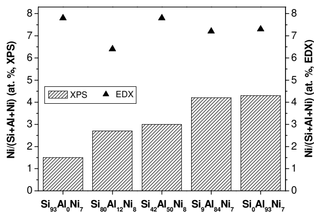
Figure 6: XPS (left axis, striped bars) and EDX (right axis, filled triangles) Ni/(Ni + Si + Al) atomic ratios for catalysts as a function of the Al 2 O 3 weight loading.
