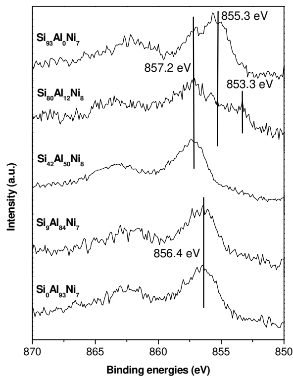
Figure 5: Ni 2p3/2 XPS spectra of Si x Al y Ni z samples.
