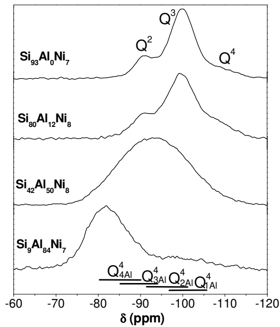
Figure 1: ^{29}\text{Si} CP-MAS NMR spectra of \text{Si}_x\text{Al}_y\text{Ni}_z samples.
