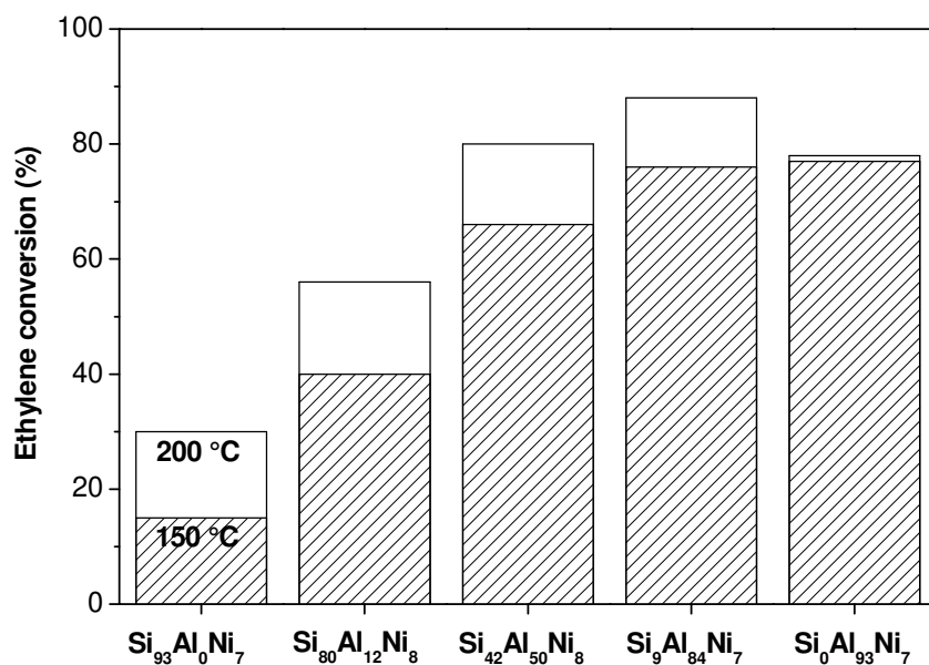
Figure 8: Ethylene conversion at 150 °C (striped bars) and 200 °C (empty bars) over the Si x Al y Ni z catalysts.
