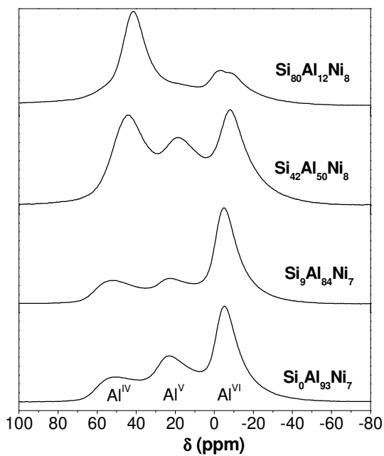
Figure 2: ^{27}\text{Al} MAS NMR spectra of \text{Si}_x\text{Al}_y\text{Ni}_z samples.
