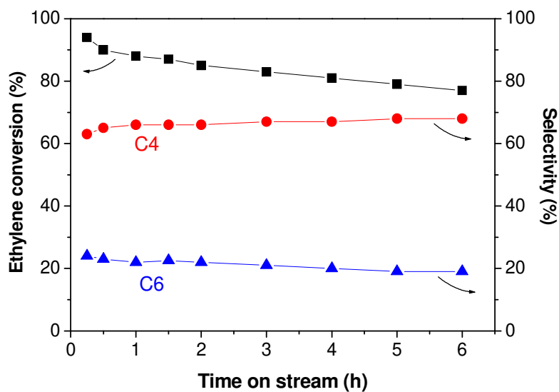
Figure 9: Ethylene conversion and C4/C6 selectivity vs. time on stream at 200 °C over the \text{Si}_9\text{Al}_{84}\text{Ni}_7 catalyst.
