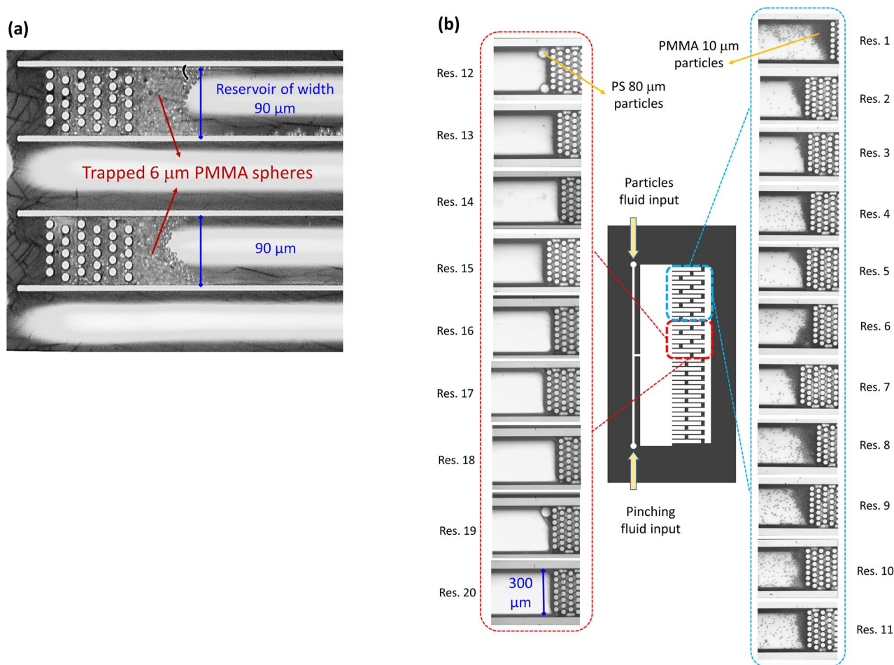
Figure 4. Particle trapping and sorting on-chip. (a) Trapping of monodisperse population of particles, consisting of standard PMMA particles of diameter 6 \mu\text{m} . (b) Sorting and trapping of polydisperse population (PMMA 10 \mu\text{m} and PS 80 \mu\text{m} standard particles) into multiple different reservoirs.
