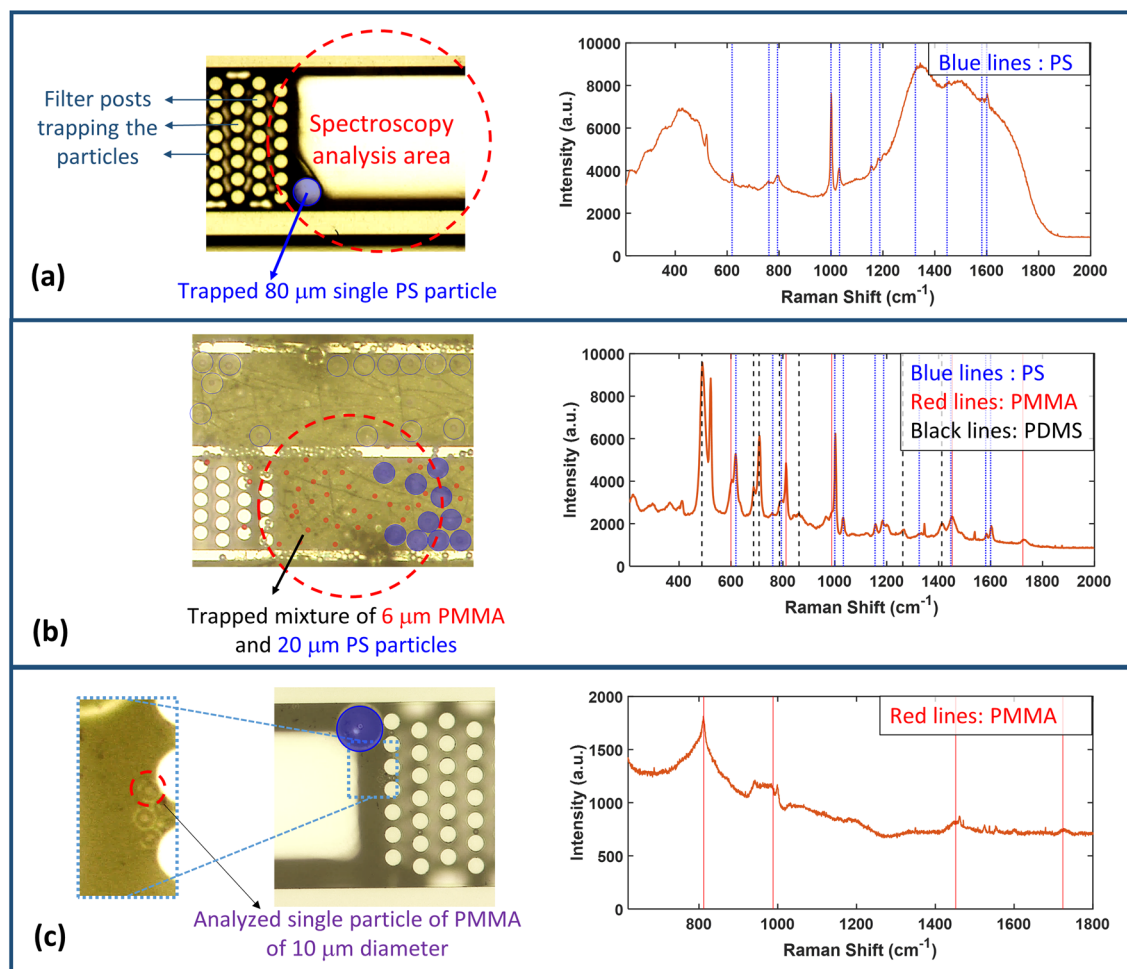
Figure 5. Raman spectrometer and Raman microscope measurements. (a) A microscope image of the chip reservoir containing a trapped PS particle of diameter 80\ \mu\text{m} , along with the obtained spectrum for this particle using the Raman spectrometer. (b) A microscope image of the chip reservoir containing a mixture of 6\ \mu\text{m} PMMA particles and 20\ \mu\text{m} PS particles, along with the obtained spectrum for this mixture using the Raman spectrometer. (c) A microscope image of the chip reservoir containing a number of particles, where only one particle is selected and analyzed (PMMA 10\ \mu\text{m} ) using the Raman microscope with the help of the small-spot size of 1\ \mu\text{m} . (a–c) Dashed-line red circles denote the area of the incident light spot for the analysis.
