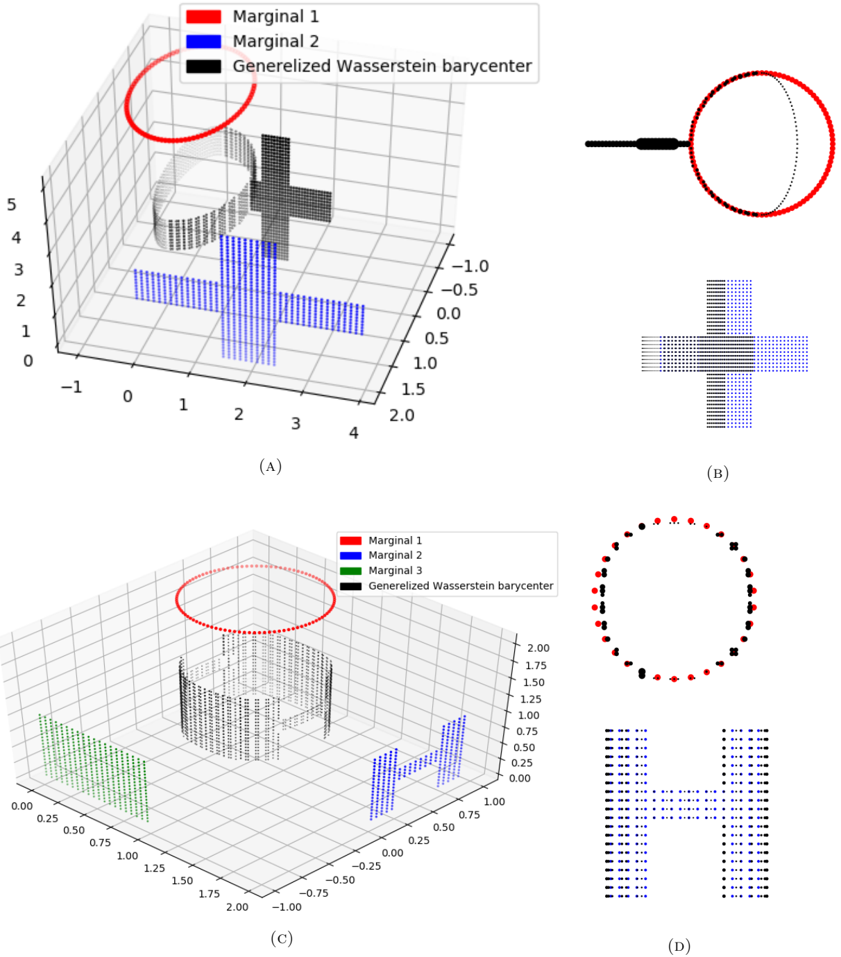
FIGURE 7. Generalized barycenters between disagreeing 2d distributions. Each line corresponds to an experiment. On the left, the three dimensional barycenter \nu (black dots) between the original two dimensional distributions \nu_i (colored dots, each color corresponding to a different i ). On the right, for each i , we show the superposition of P_i \# \nu (black) and \nu_i .
