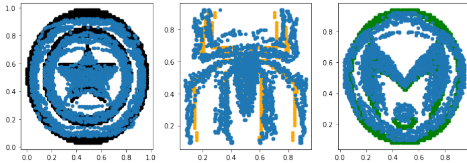
FIGURE 8. Generalized Wasserstein Barycenter (in blue) between three dots distributions representing logos of super heroes (Captain America in black, Scarlet Witch in green and Spiderman in orange), with P_1 = \begin{pmatrix} 1 & 0 & 0 \\ 0 & 1 & 0 \end{pmatrix} , P_2 = \begin{pmatrix} 0 & 1 & 0 \\ 0 & 0 & 1 \end{pmatrix} and P_3 = \begin{pmatrix} 1 & 0 & 0 \\ 0 & 0 & 1 \end{pmatrix} . Top: three marginals and generalized barycenter with a fixed number of masses (2000 points here), obtained by optimizing the mass locations but not the weights, as described in [9]. Bottom: projections P_i \# \gamma^* of the generalized barycenter superposed with the \nu_i .
