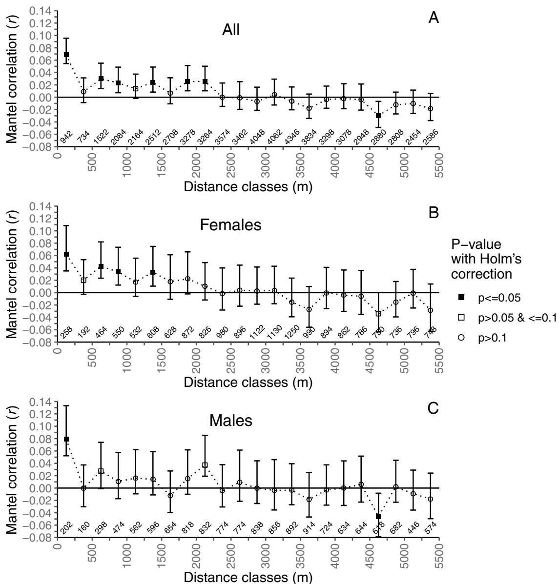
Fig. 3 Mantel correlogram considering (a) all individuals ( N=280 ), (b) only females ( N=148 ) and (c) only males ( N=130 ), with distance classes following a 250-m step. Mantel tests were performed with 10,000 permutations and 95% confidence intervals from 1,000 boot-
