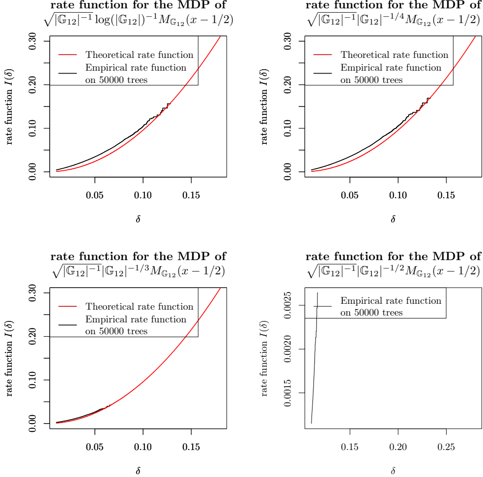
FIGURE 1. Exact and empirical rate functions for the moderate deviation principles of |\mathbb{G}_n|^{-1/2} b_n^{-1} M_{\mathbb{G}_n}(x - 1/2) . In the first three figures, one can see that empirical rate function fit well the exact rate function. The differences can be explained from the fact that the sample size is not large enough to generate enough large deviation events. In the last figure, one can see that the empirical rate function is reduced to 0. This is due to the fact that the speed considered here is valid only in the critical case, not in the subcritical case.
