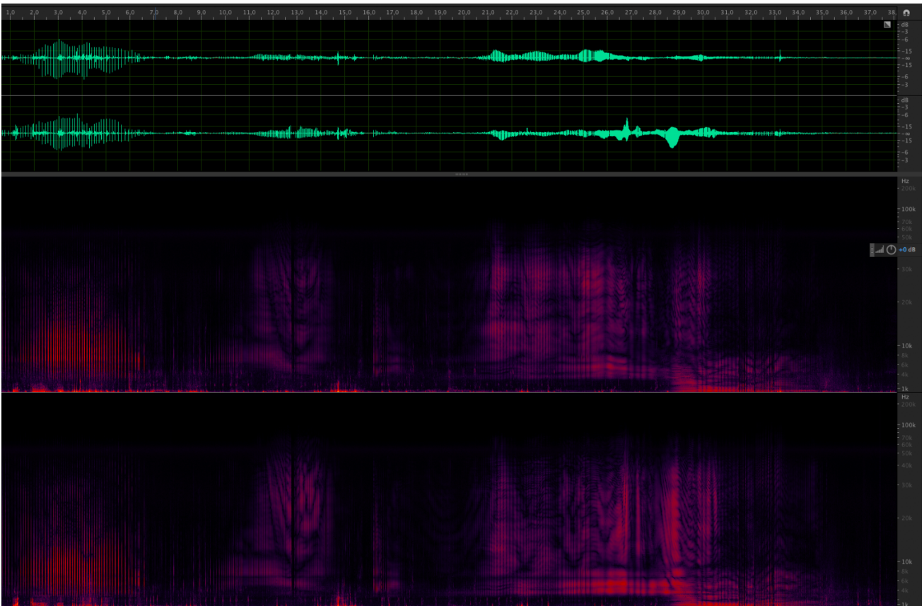
Figure 5. Spectrogram of Physeter macrocephalus , P.m. in near field measured by our system showing click trains up to 50 kHz. Stereo recording of the 14 th of April 2018, at 300 kHz Sampling Rate, 16 bits, hydrophones CR57 (Cetacean Research Tech., USA). Graphic with the help of M. Mercier (TripinLab).
