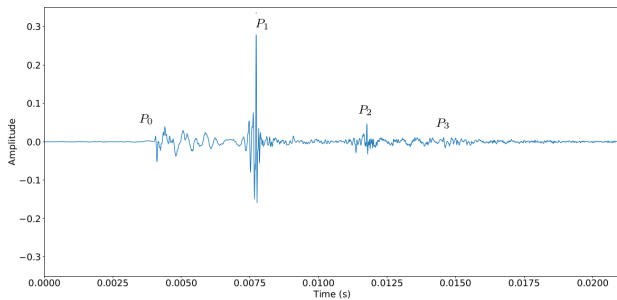
Figure 2. Example of a Sperm whale click demonstrating its multipulsed structure P_0 , P_1 , P_2 . The nominal IPI is the time lapse between P_1 to P_2 .
