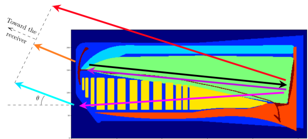
Figure 1. Pulse path in the head of the Sperm whale in the leaky bent horn model. The spermaceti is in the green volume.
