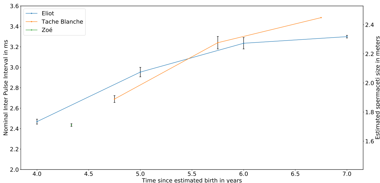
Figure 7. Measurements of the nominal IPI of three youngs, over 3 years for two of them, showing their growth. Respective birth dates are: Tache Blanche June 2011; Eliot March 2011; Zoé December 2013.
