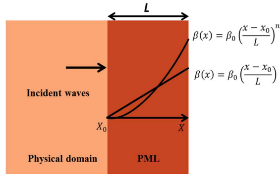
Fig. 2 Evolution of the damping functions in PML subdomain
