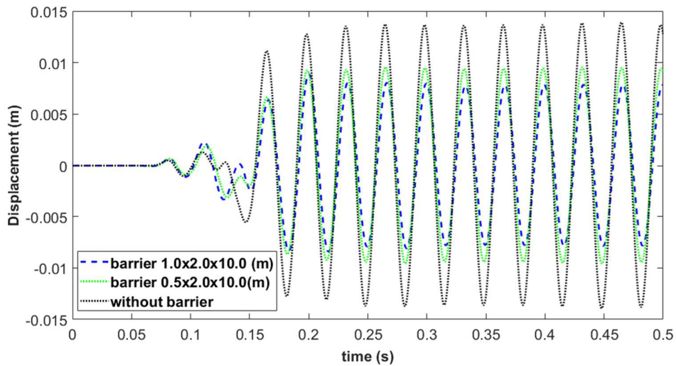
Fig.19 Time histories of the displacement at the recording point in the case of wave barriers with different depths, compared to the results obtained without barrier.
