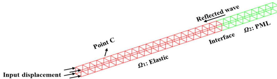
Fig.8 Semi-infinite elastic 3D bar subjected to horizontal displacement
