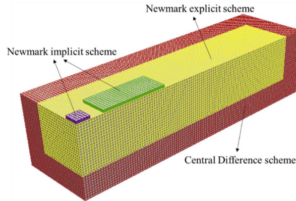
Fig.13 Different time integration schemes for different subdomains
