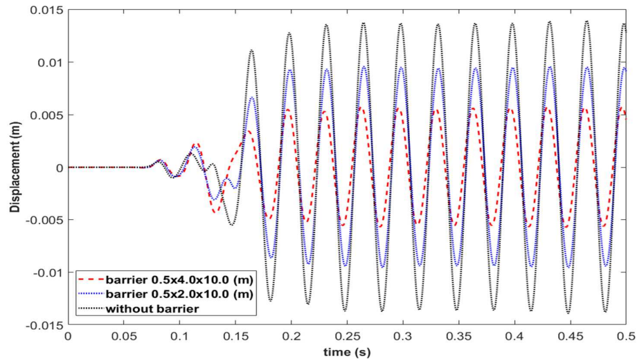
Fig.18 Time histories of the displacement at the recording point in the case of wave barriers with different widths, compared to the results obtained without barrier
