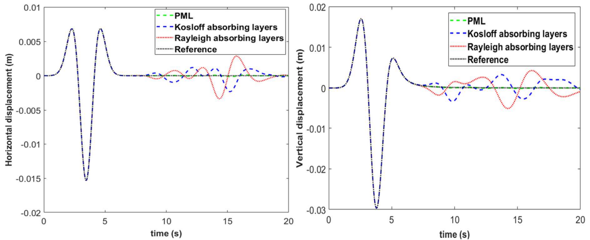
Fig.7 Vertical and horizontal displacements at the recording point using different absorbing layers (the length of the three absorbing layers is equal to 50m)
