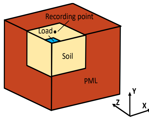
Fig.10 3D Lamb's test modeled using PML: quarter model of a PML-truncated semi-infinite homogeneous media subjected to a concentrated force
