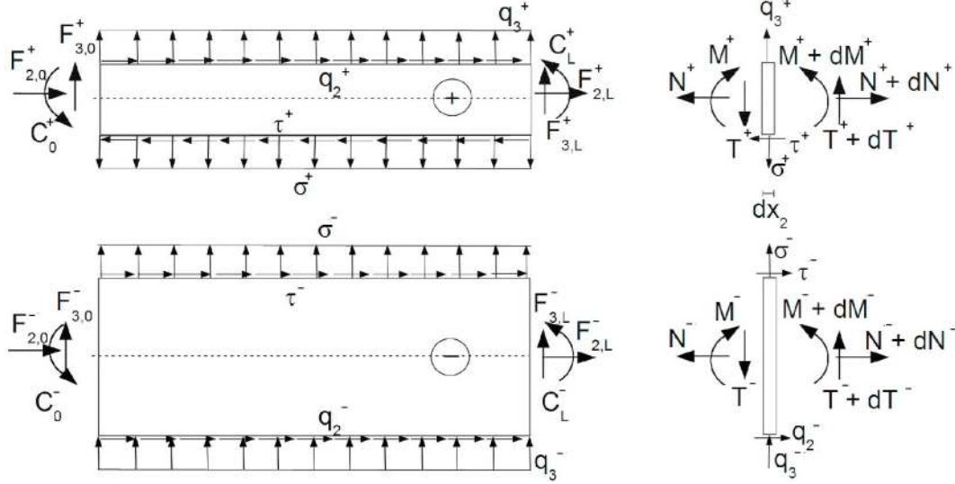
Fig. 2. Free body diagrams of the two adherent beams (left), and of two infinitesimal elements of the beams (right).
