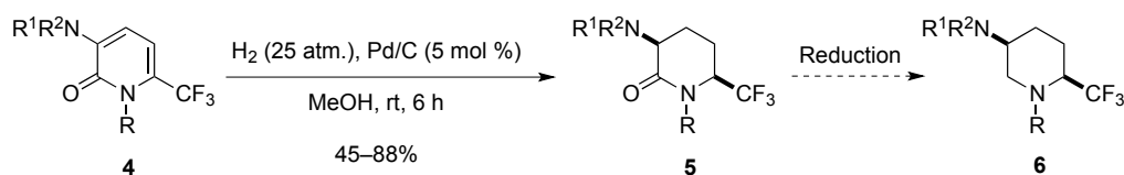
Scheme 4. Hydrogenation of trifluoromethylpyridinones.
