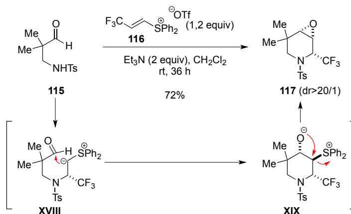
Scheme 35. Synthesis of \alpha -trifluoromethylpiperidino-epoxides.
