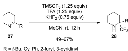
Scheme 13. Synthesis of \alpha,\alpha -disubstituted piperidines.
