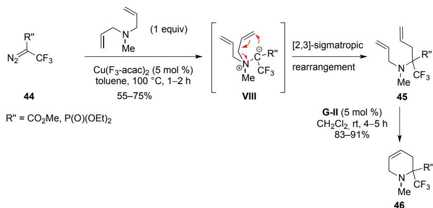
Scheme 18. Synthesis of \alpha,\alpha -disubstituted piperidines from trifluorodiazo derivatives.
