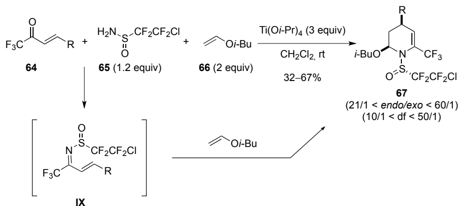
Scheme 22. Aza Diels-Alder reaction with 1-azadienes.
