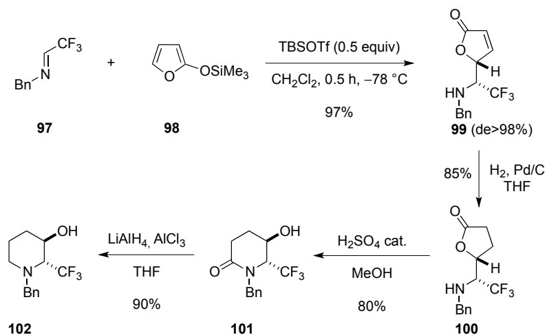
Scheme 31. Synthesis of an \alpha -trifluoromethylpiperidine by lactamization.
