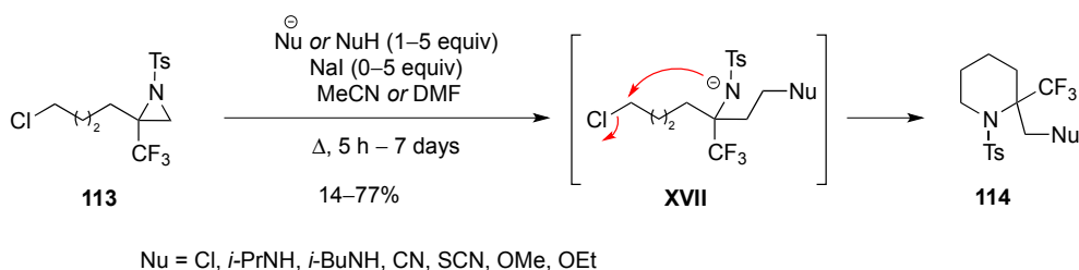
Scheme 34. Synthesis of \alpha -trifluoromethylpiperidines from trifluoromethylaziridines.
