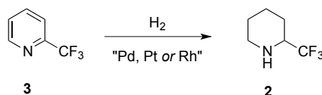
Scheme 3. Hydrogenation of \alpha -trifluoromethylpyridine.
