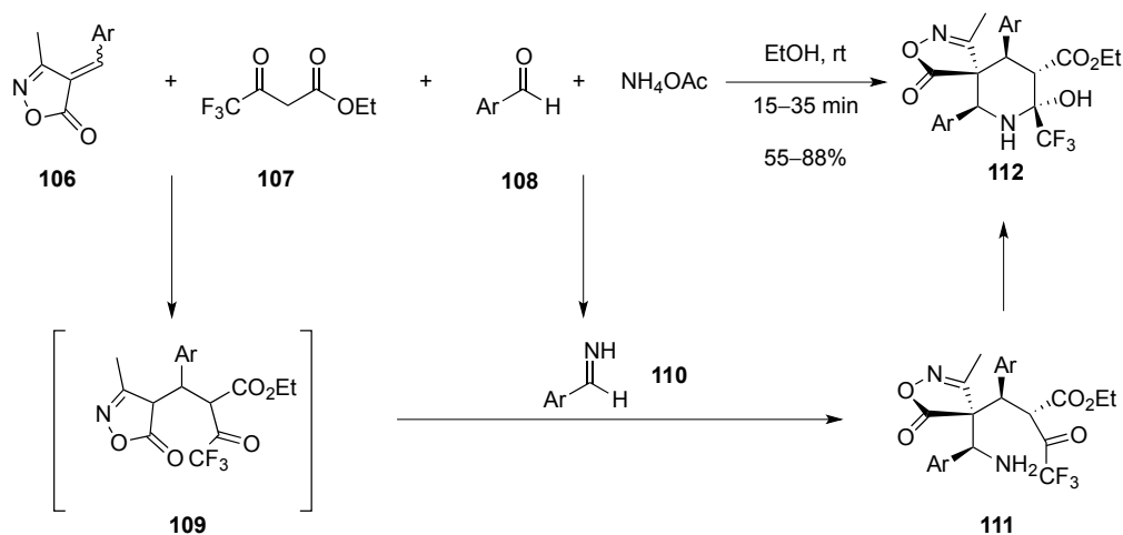
Scheme 33. Synthesis of highly substituted \alpha -trifluoromethylpiperidines.
