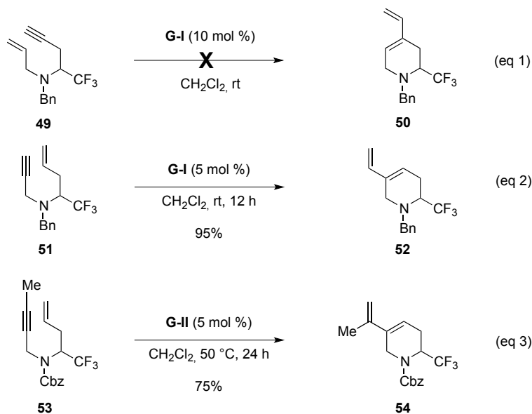
Scheme 20. Cont.
