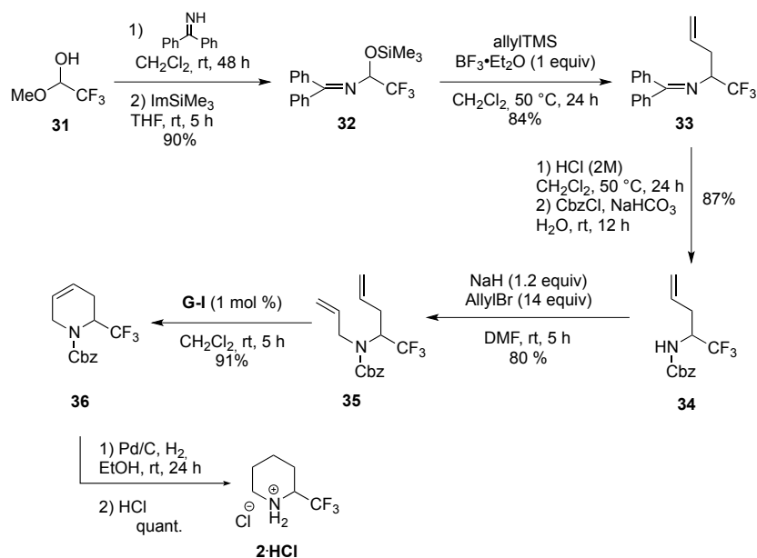
Scheme 15. Synthesis of \alpha -trifluoromethylpiperidine from trifluoromethylhemiacetal.
