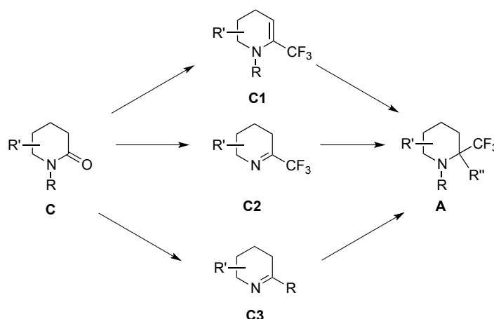
Scheme 5. Synthesis of \alpha -trifluoromethylpiperidines from \delta -lactams.
