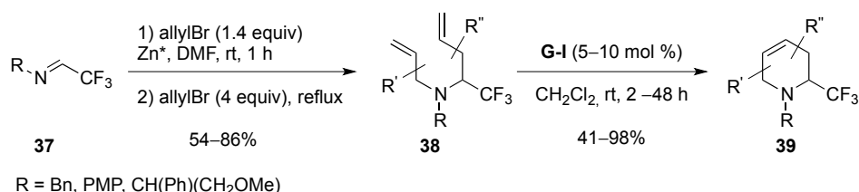
Scheme 16. Synthesis of \alpha -trifluoromethylpiperidines from trifluoromethylimines.
