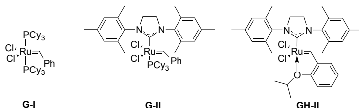
Figure 1. Catalysts for olefin metathesis.
