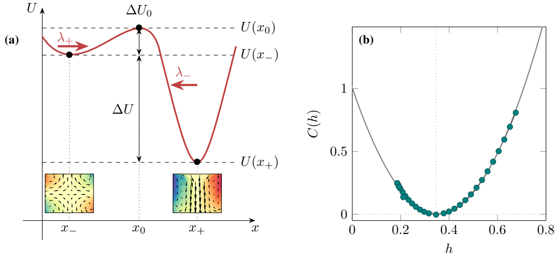
Figure 11. (a) Energy landscape picture of the bifurcation. The von Kármán flow evolves, as would a Brownian particle, between two potential wells of different depths U(x_-) and U(x_+) separated by energy barriers \Delta U_0 or \Delta U + \Delta U_0 depending on the nature of the transition. (b) Multifractal spectrum in the von Kármán flow computed using numerical simulations by Hugues Faller. The data point are in green, the dotted line is a parabolic fit allowing extrapolation towards C(h) = 3 which cannot be accessed with our limited data set. [Figure adapted from Faller et al. (2021)]
