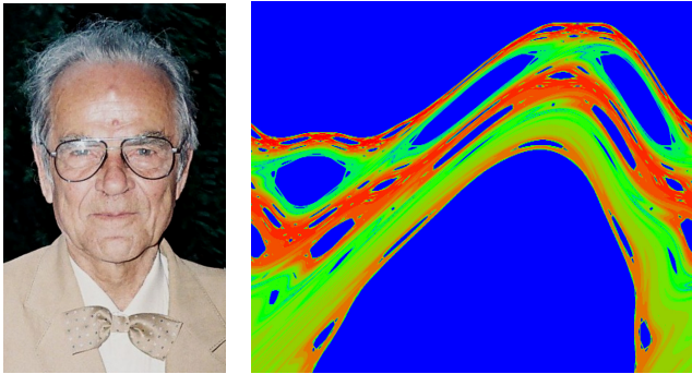
FIG. 3. Left: Boris Chirikov, Toulouse, June 6, 1998. Photo by D. L. Shepelyansky. Right: Amplitude of the eigenstate of the Ulam approximate of Perron-Frobenius operator of the Chirikov standard map at K = 0.971635406 ; amplitude is proportional to color with maximum for red and zero for blue; upper part of phase plane is shown for the range 0 < \frac{x}{2\pi} \leq 1 , 0 < \frac{p}{2\pi} \leq 0.5 . From Frahm et al , 2010.
