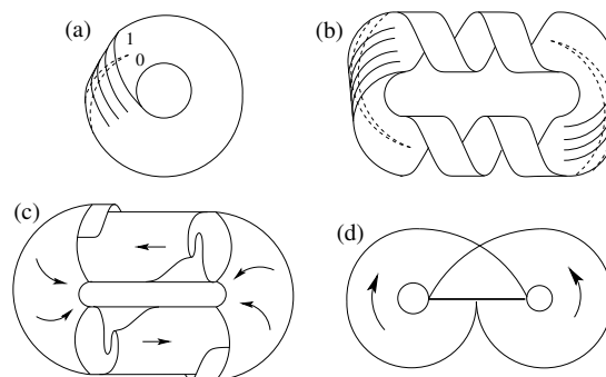
FIG. 14. Branched manifolds describing (a) Rössler, (b) periodically driven Duffing, (c) van der Pol attractors, and (d) Lorenz attractors and for particular parameter values. Redrawn from The topology of chaos , p. 133, (Wiley, 2003).
