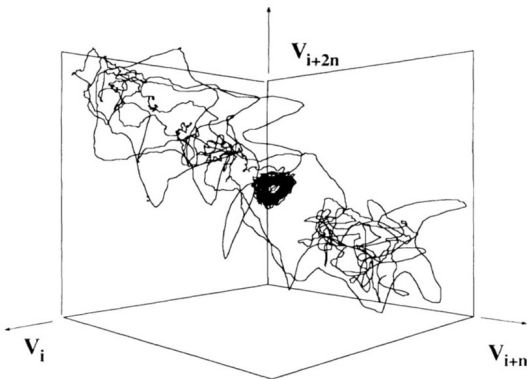
FIG. 15. Trajectory of a chaotic transient ending in a periodic attractor. Reproduced with permission from Phys. Rev. Lett. 59, 2891 (1987). Copyright 1987, American Physical Society.
