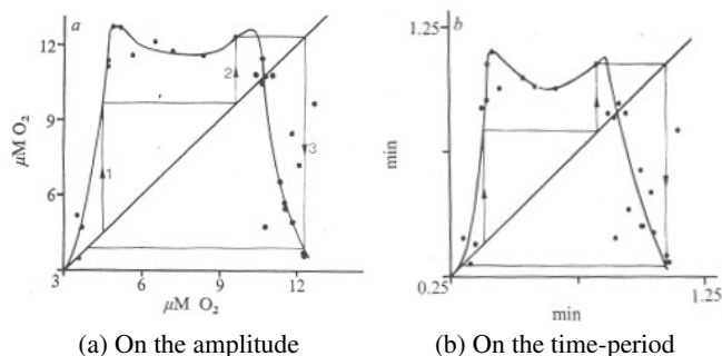
FIG. 10. a) Next-amplitude map of oscillations of O_2 from Fig. 9(b); b) same type of plot for the oscillation periods. Trajectories with arrows were drawn to show that the transition function allow the period 3. Reproduced with permission from Nature 267, 177 (1977). Copyright 1977, Springer Nature.
