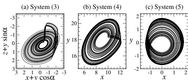
FIG. 4. The chaotic attractor obtained after some simplifications of the original equations. Parameter values for system (3): \delta = \varepsilon = 0.03 . For system (4): a = 0.2 , b = 0.2 , c = 5.7 . For system (5) b = 0.275 and c = 0.2 and initial conditions are x_0 = 1 , y_0 = -1.4 and z_0 = -0.4 .
