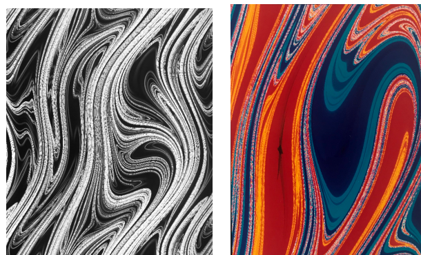
FIG. 12. Fractal basin boundary and the basins of attraction of the forced damped pendulum equation (14). Parameter values: v = 0.1 , \omega = 1 , and f = 2 . Reproduced with permission from Science 238, 632 (1987). Copyright 1987, American Association for the Advancement of Science.
