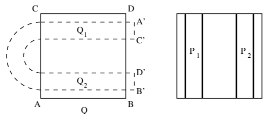
FIG. 1. Smale's horseshoe map. A global diffeomorphism maps the square Q into the region bounded by dotted lines with G(A) = A' , etc. Each component P_1 and P_2 of g^{-1}(g(Q) \cap Q) is such that g is a linear map with g(P_i) = Q_i ( i = 1, 2 ).
