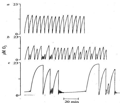
FIG. 9. Simple periodic (a), chaotic (b) and bursting (c) oscillations of O_2 in the peroxidase-oxidase reaction. Reproduced with permission from Nature 267, 177 (1977). Copyright 1977, Springer Nature.
