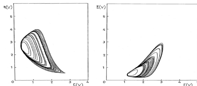
FIG. 11. "Chaotic" orbits yielded by the analog computer at Yoshisuke Ueda's laboratory in 1978 by using the model (13). Parameter values: p \approx 90 , \phi \approx 0.048 , and m \approx 3.44 . Figures reproduced from the Ichiro Tsuda's Master thesis, Kyoto University, 1979.
