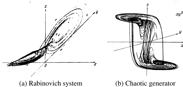
FIG. 8. Phase portraits of two strange attractors created on an analog computer produced by (a) the Rabinovich system (11) and (b) the electronic chaotic generator. Reproduced with permission (a) from Zhu. Eksp. Teor. Fiz., 74, 1366 (1978) and (b) from Dok. Akad. Nauk SSSR. 239, 301 (1978). For both, copyright 1978, Russian Academy of Sciences.
