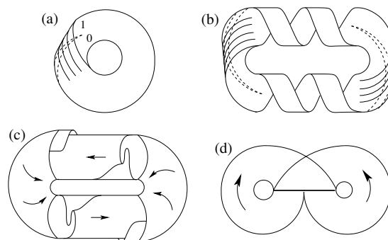
FIG. 14. Branched manifolds describing (a) Rössler, (b) periodically driven Duffing, (c) van der Pol attractors, and (d) Lorenz attractors and for particular parameter values. Redrawn from The topology of chaos , p. 133, (Wiley, 2003).
