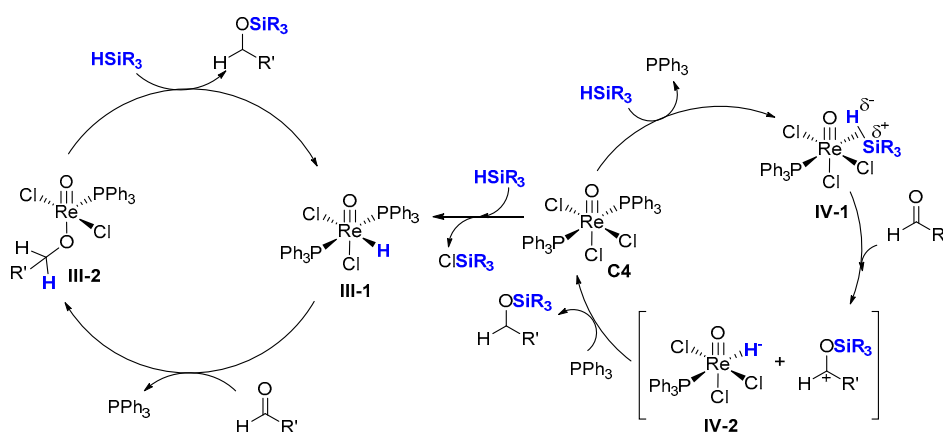
Scheme 5. The \sigma -bond metathesis pathway involving the isolated hydride intermediate \text{Re}(\text{O})\text{Cl}_2\text{H}(\text{PPh}_3)_2 ( left ). The pathway involving a \eta^2 -silane complex ( right ).
