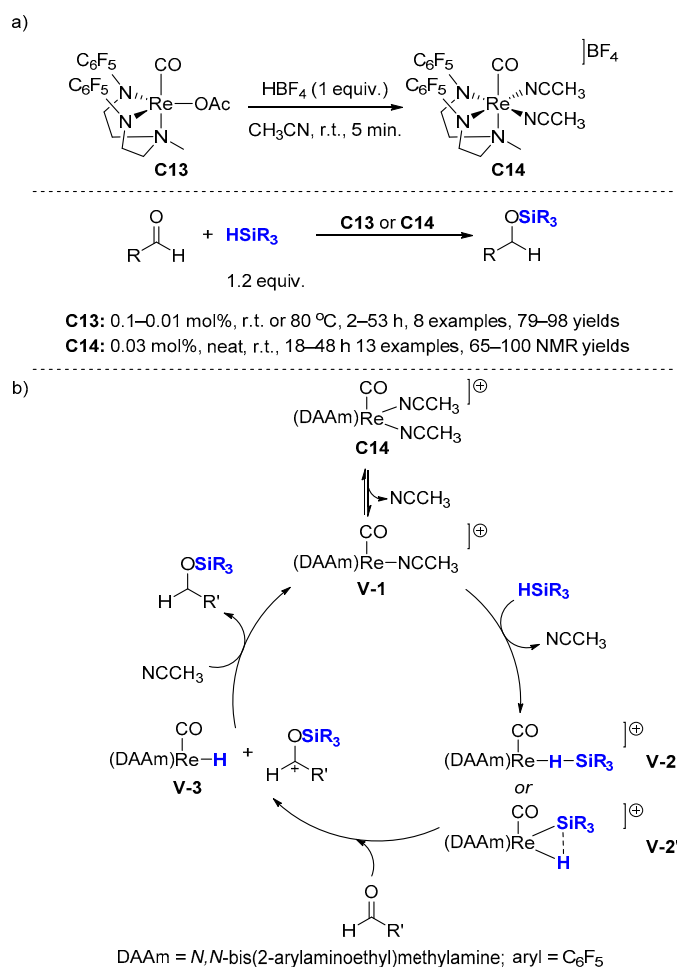
Scheme 7. Cationic rhenium complex catalyzed hydrosilylation of aldehydes. (a) Scope of the reaction; (b) Proposed mechanism.
