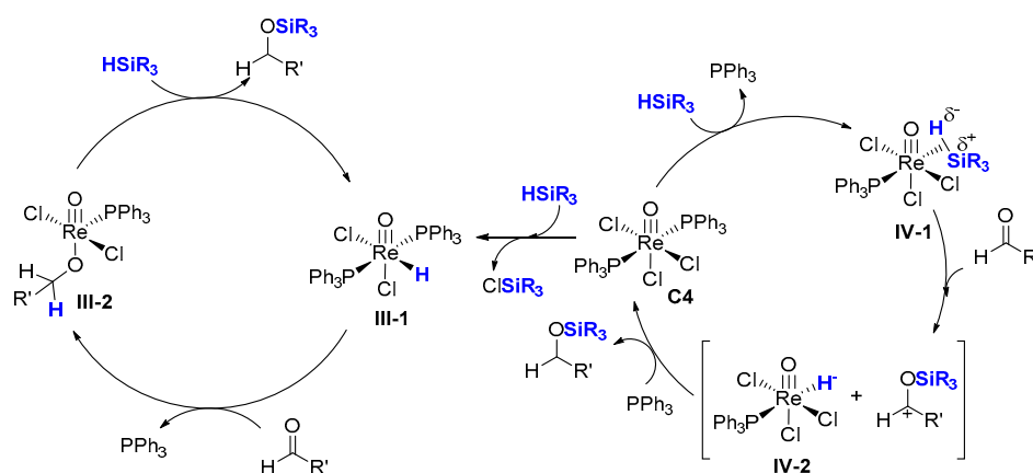
Scheme 5. The σ-bond metathesis pathway involving the isolated hydride intermediate Re(O)Cl 2 H(PPh 3 ) 2 (left). The pathway involving a η 2 –silane complex (right).
