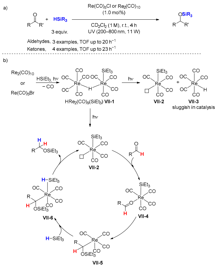
Scheme 9. Hydrosilylation of carbonyls via \text{Re}(\text{CO})_5\text{Cl} photolysis (a) and proposed mechanism (b).
