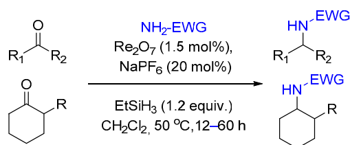
Scheme 12. Direct reductive amination of ketones with electron-deficient amines using \text{Re}_2\text{O}_7/\text{NaPF}_6 catalyst system.
