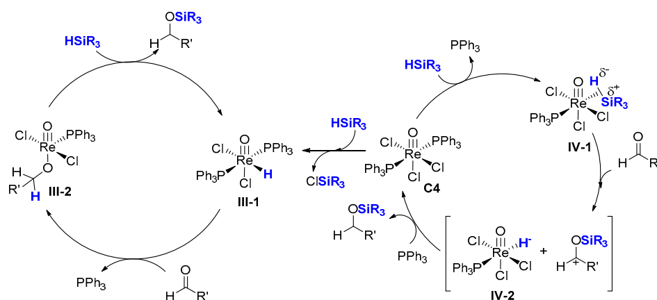
Scheme 5. The \sigma -bond metathesis pathway involving the isolated hydride intermediate Re(O)Cl 2 H(PPh 3 ) 2 (left). The pathway involving a \eta^2 -silane complex (right).
