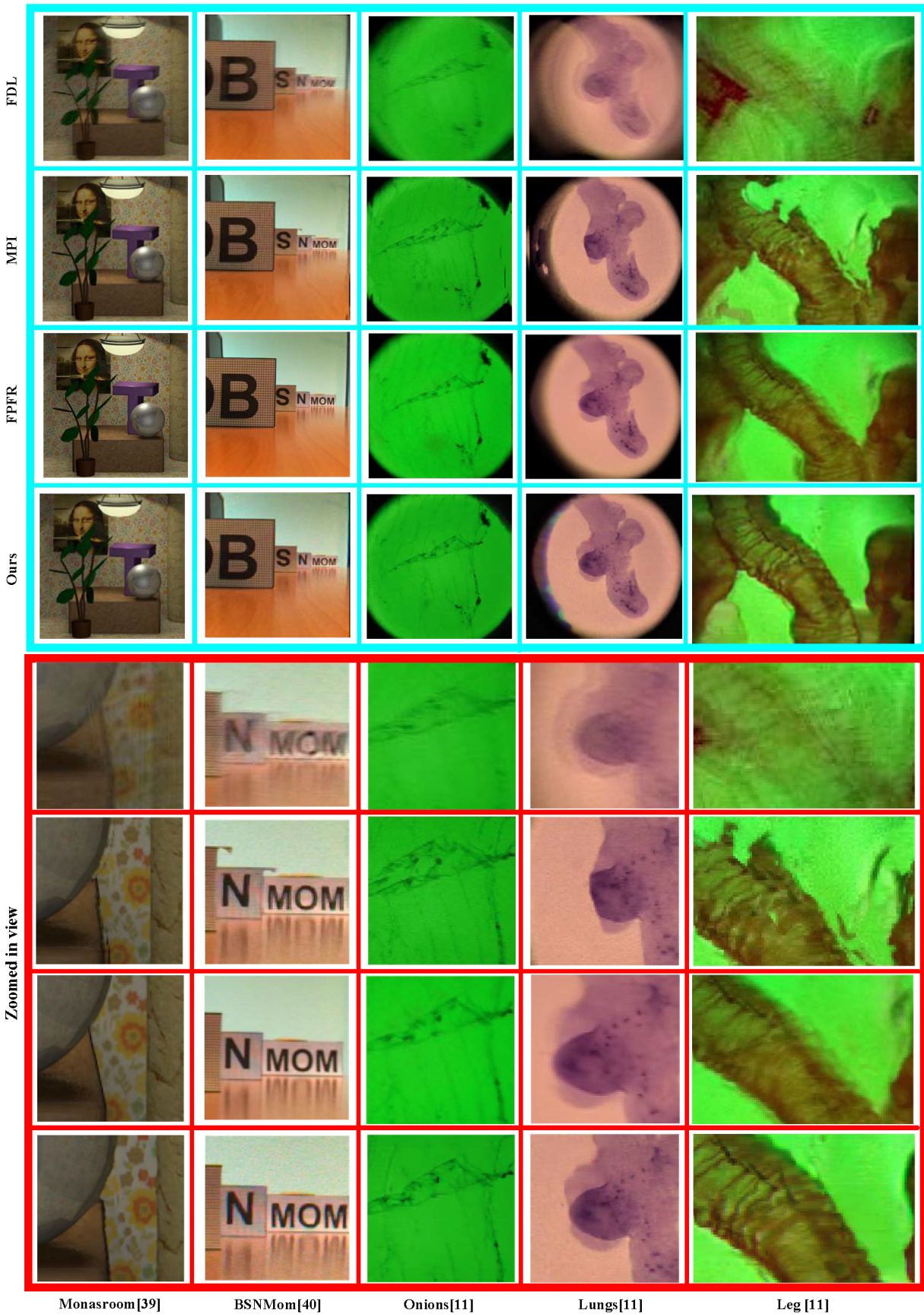
Fig. 7. Visual comparison of extrapolation results obtained with four different methods, FDL [28], MPI-based extrapolation[30], FPF-based extrapolation [37], and ours, with a 4X larger baseline. For five light field datasets, we show that our extrapolation method can generate much better results than the methods in [28], [30] and [37]. From the zoomed views, we can see that the FDL method may introduce blur, and the MPI method may generate wrong textures if regions of ambiguous or repetitive texture are assigned with inaccurate opacity weights when using the multiple layer representation. The FPF method may introduce blur when the depth estimation is not accurate enough, e.g. in the scene of Onions and Leg
