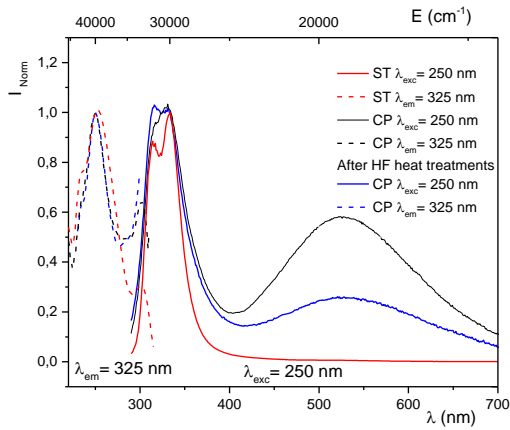
Figure S17- Luminescence of Ce-doped CaSnF- compound ; sealed tube (red curves ; coprecipitation route after synthesis : black curves ; after heat treatment : bleu curves
