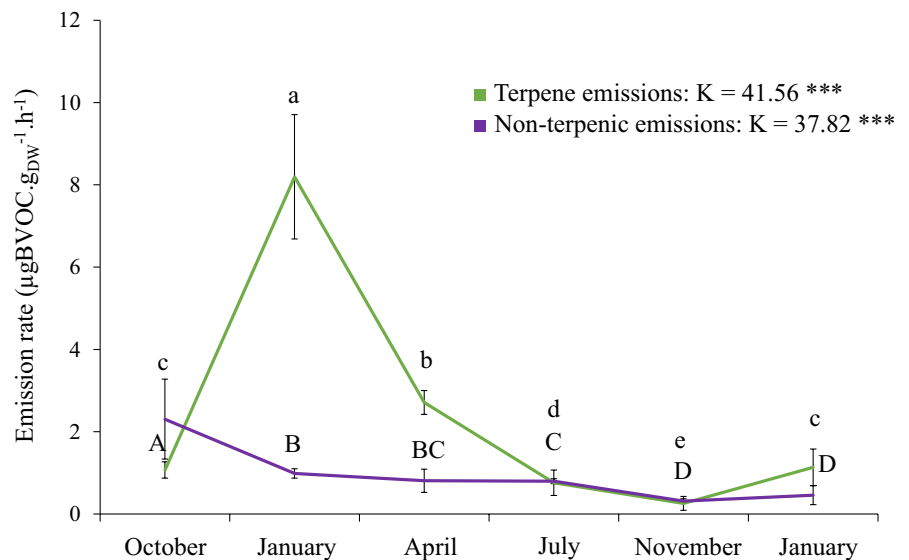
FIGURE 2 Evolution of nonterpenic (purple line) and terpenic emissions (green line) from Pinus halepensis litter through the decomposition experiment. Values are mean \pm SD; n = 7 . K-values and associated P-values (***) for P < 0.001 are indicated. Different letters denote significant differences between decomposition times with a > b > c > d > e (Fisher LSD tests)
