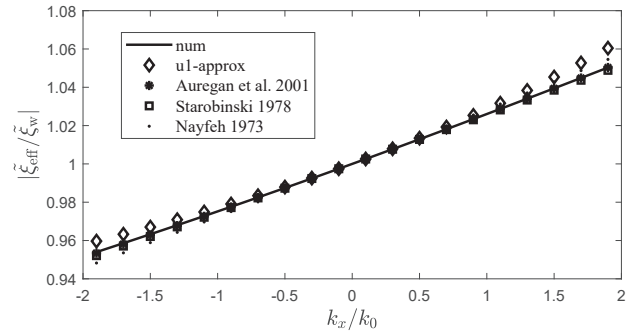
Figure 7. Effective displacement as a function of the normalized streamwise wavenumber k for M_\infty = 0.1 , 500 Hz, and exponential mean flow.
