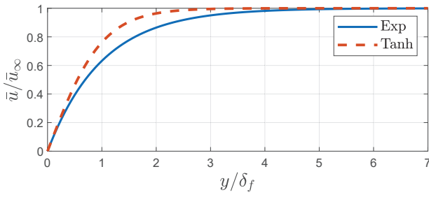
Figure 5. Used flow boundary layer profiles.
