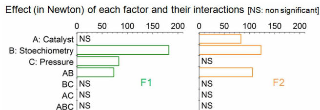
Figure 5. Histograms of the effects of factors and interactions (in newtons) for each response (F1: force at break at first welding; F2: at second welding) [NS: non significant].
