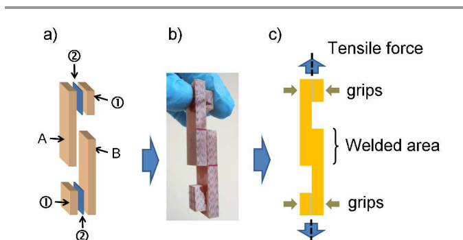
Figure 4. a) Exploded view of lapshear specimens ① shims, ② glue, A, B: composite adherands; welding is performed at the central part. b) Aspect of 2:1-Zn vitrimer composites slabs after welding, c) principle of the lap-shear test.
