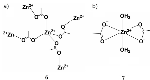
Figure 3. Reference compounds used in EXAFS studies. a) In compound 6: (ZnAc 2 ) Zn 2+ is tetraordinated with bridging acetate ligands. b) In compound 7 (ZnAc 2 •2H 2 O) Zn 2+ is hexacoordinated with bidentate acetate ligands and water.
