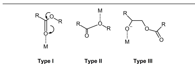
Figure 6. Possible complexation modes of a \beta -oxy ester group with a metal M. Experimental data suggest the presence of type I and type III complexation.
