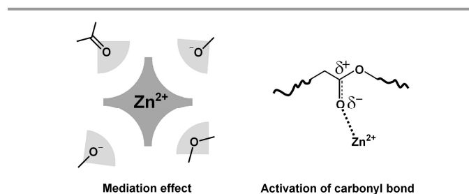
Figure 7. The two main actions of zinc as a catalyst in epoxy-acid vitrimer network: mediation effect and ester activation designed from EXAFS and IR spectroscopy observations.
