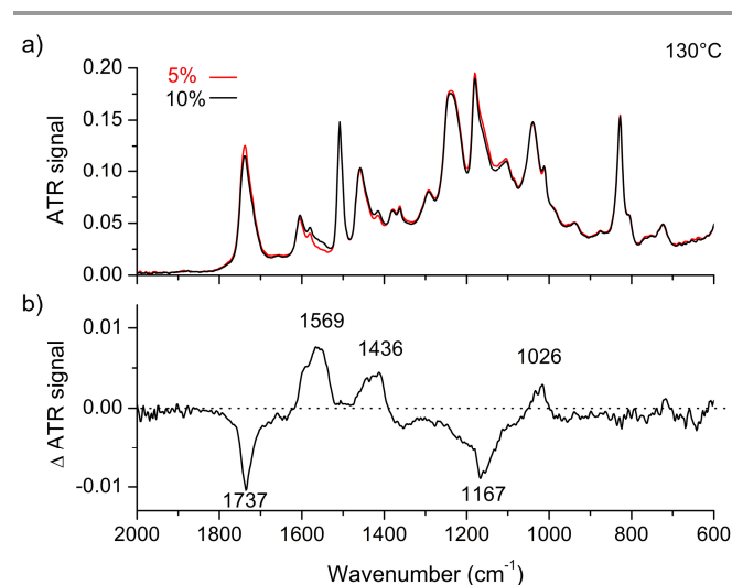
Figure 5. a) ATR-IR spectra of 5 mol% Zn-catalyzed epoxy vitrimer (red) and 10 mol% Zn-catalyzed vitrimer (black). b) ATR-IR spectrum difference A(10\%) - A(5\%) .
