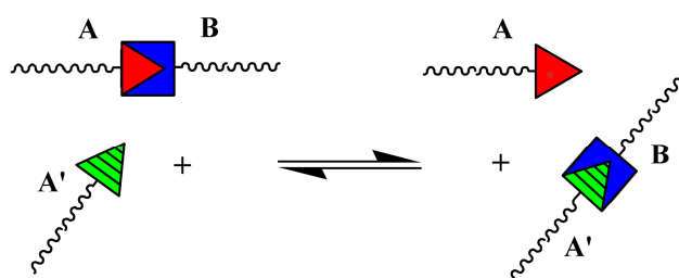
Figure 1. Basic view of an exchange reaction.
