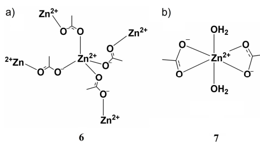
Figure 3. Reference compounds used in EXAFS studies. a) In compound 6: (ZnAc 2 ) Zn 2+ is tetraordinated with bridging acetate ligands. b) In compound 7 (ZnAc 2 ·2H 2 O) Zn 2+ is hexacoordinated with bidentate acetate ligands and water.
