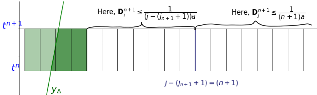
Figure 3: Illustration of the OSL bound (3.16).
