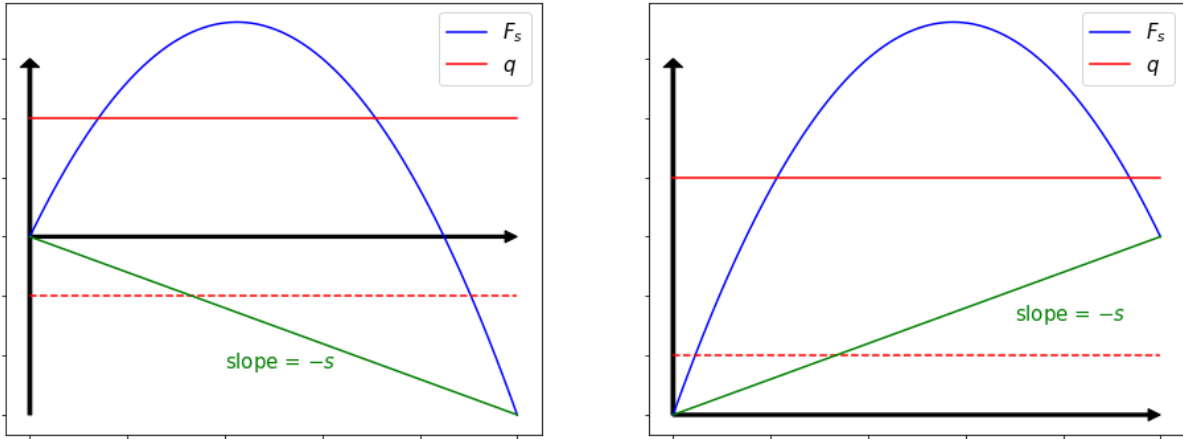
Figure 1: Illustration of Assumption (2.3)
