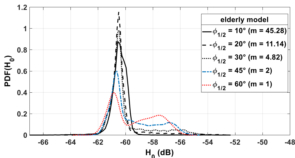
Figure 8. PDFs of H_0 for different values of \phi_{1/2} with young model (a) and with elderly model (b).
