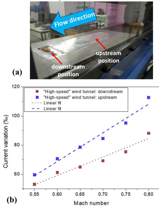
Fig. 7. (a) Experimental setup of the micro-sensor inside the high-speed wind tunnel in S8Ch at ONERA Meudon (b) Results: measured time-averaged current variation with Mach number, for two different positions of the micro-sensor on the flat plate, upstream and downstream.
