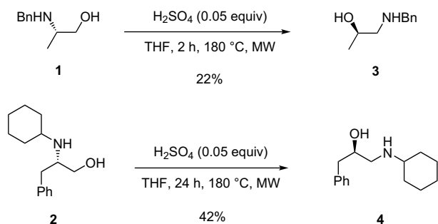
Scheme 3. Rearrangement of N -alkyl \beta -amino alcohols 1 and 2 with H_2SO_4 .
