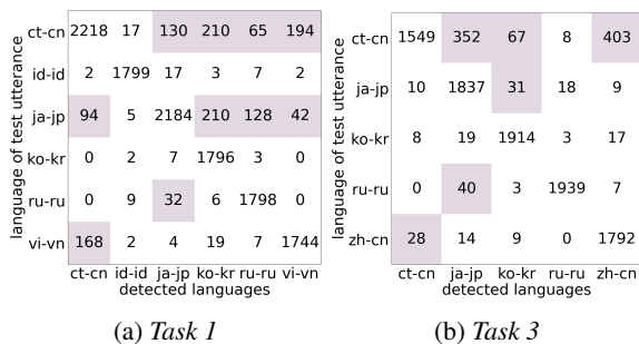
Figure 1: Confusion matrices of the submitted system on the evaluation set (number of utterances). Multiple detections are possible. Language labels are defined in Subsection 2.1. Colored numbers correspond to a high number of errors.
