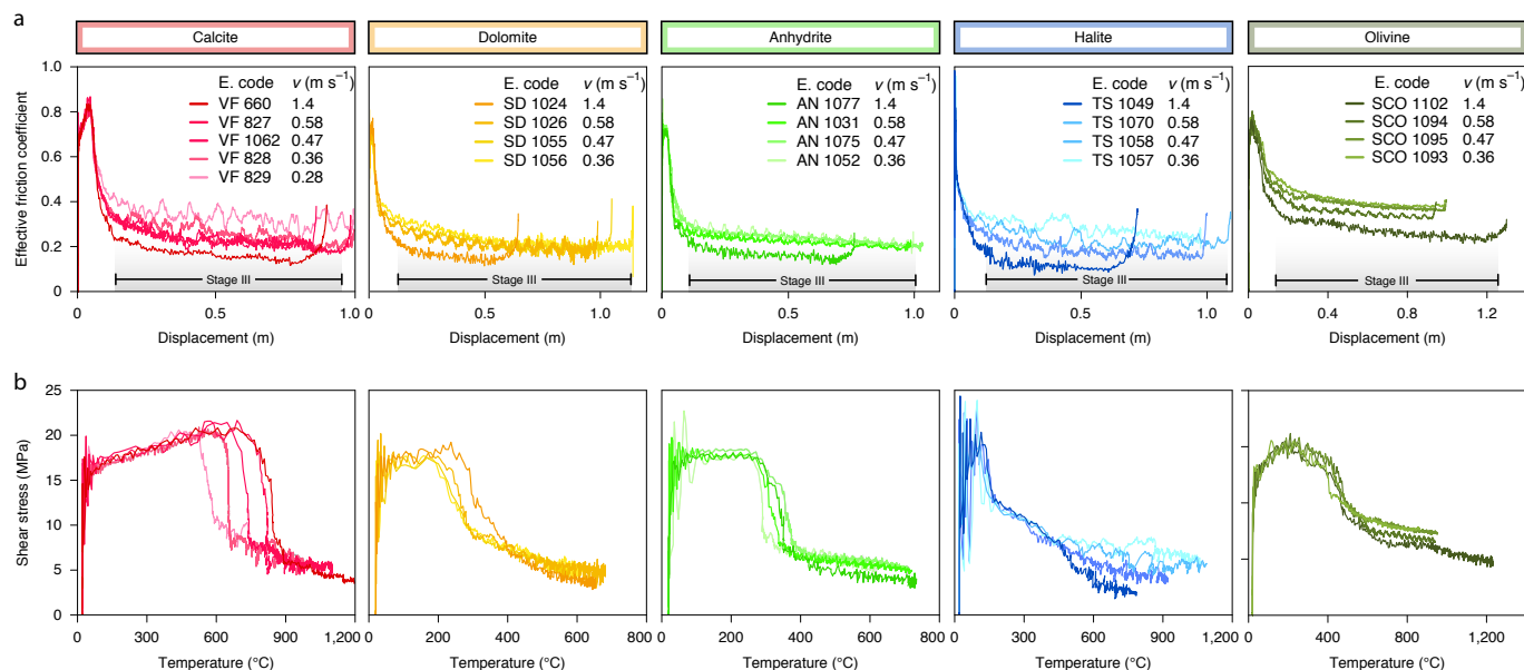
Fig. 1 | Mechanical data. a , \mu^* evolving with displacement during Stages I–IV (see text for details). During Stage III, \mu^* values are lower in experiments run at higher velocities. Each experiment terminates with partial re-strengthening during deceleration to arrest. b , Shear stress as a function of calculated temperature (up to Stage III). Note that the Stage III mechanical data of calcite, dolomite and anhydrite—and with good approximation for halite and olivine—collapse onto a single material-characteristic curve. Halite curves overlap up to a temperature of \sim 440^\circ\text{C} . E. code, alphanumeric experiment code.
