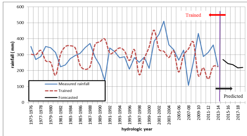
Figure 7: Expected (predicted) yearly rainfall of Central Mesaria region based on AR(1) model for hydrologic years 2014-15 to 2018-19
