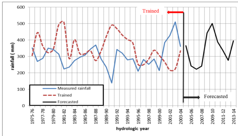
Figure 5 : Graphical comparison of AR(1) model (trained and forecasted) and the hydrologic yearly averaged rainfall (measured) of Central Mesaria
