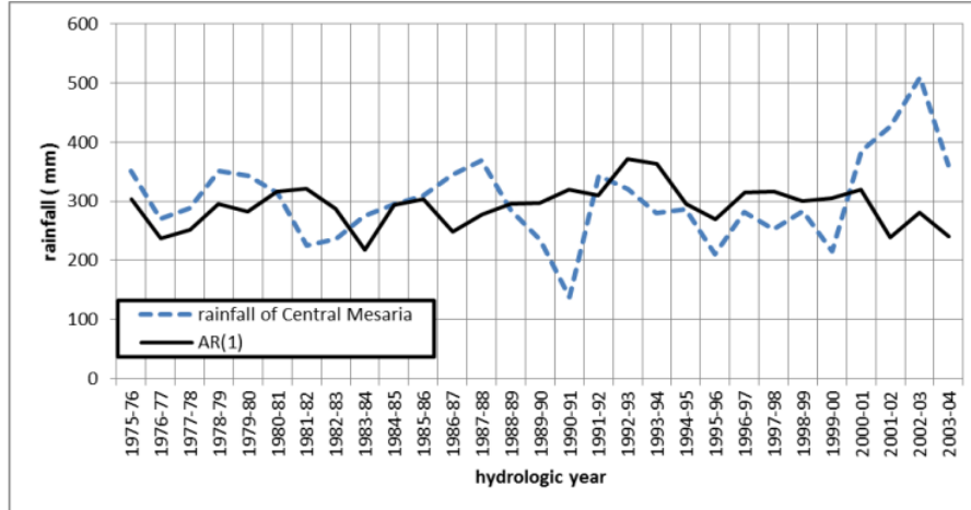
Figure 2 : Synthetically generated AR(1) model and the respective measured rainfalls of Central Mesaria for the period of hydrologic years 1975-76 to 2003- 04
