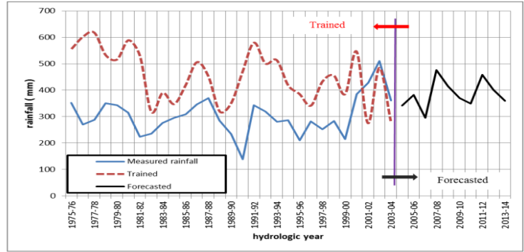
Figure 4 : Graphical comparison of Markov model (trained and forecasted) and the hydrologic yearly averaged rainfall (measured) of Central Mesaria
