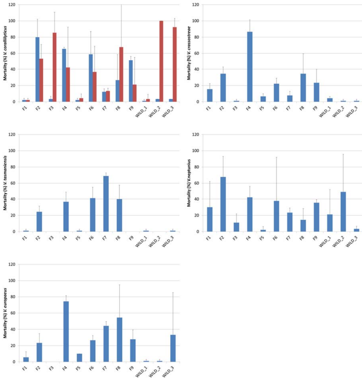
Figure 4: Mortality (% + SD among replicates) 7 days post-infection by V. coralliilyticus , V. crassostreae , V. tasmaniensis , V. neptunius , and V. europaeus for the nine families and the three wild stocks in Larval 1 (blue) and Larval 2 (in red) using a batch method. Due to the absence of difference in mortality between the control and experimental infection using bacteria, data are not showed for V. harveyi in both larval trials, and for Larval 2 except for V. coralliilyticus .
