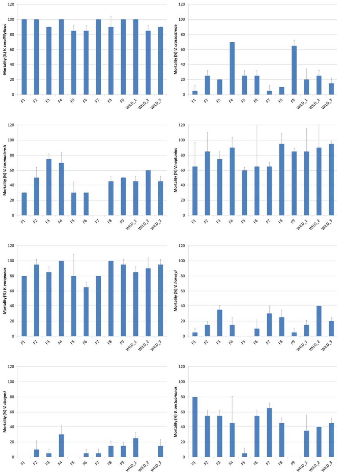
Figure 3: Mortality (% + SD among replicates) 3 days post-injection by V. coralliilyticus , V. crassostreae , V. tasmaniensis , V. neptunius , V. europaeus , V. harveyi , V. chagasi , and 13 days post-
