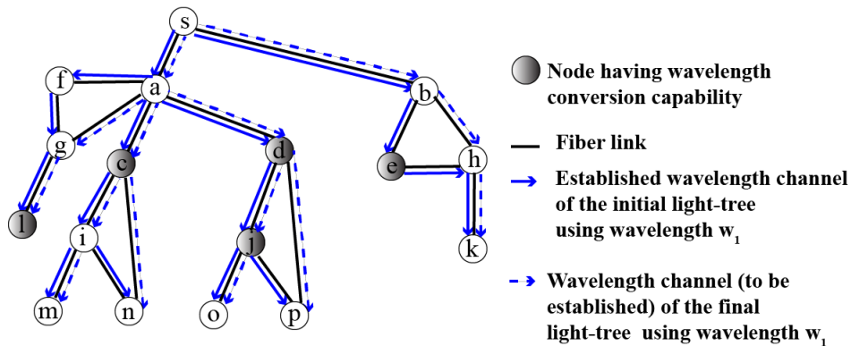
Figure 6. Instance of problem.
