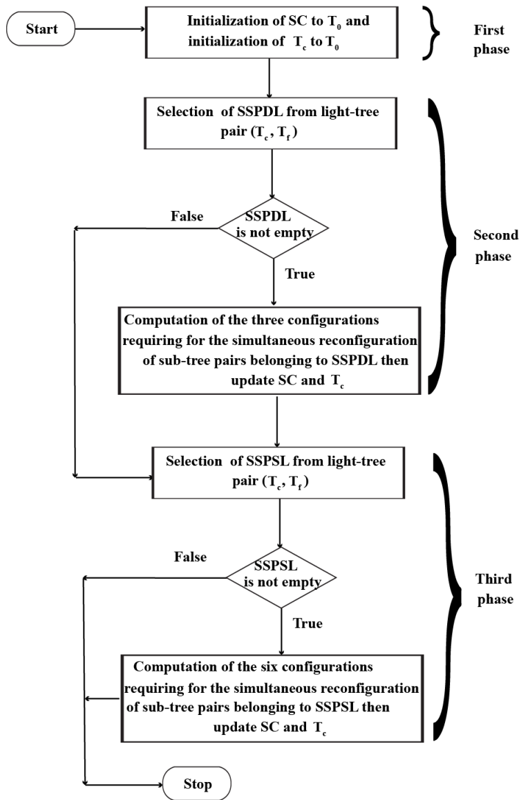
Figure 5. Flowchart of our method (i.e., Algorithm 1); SSPDL = set of sub-tree pairs with disjointed links; SSPSL = set of sub-tree pairs with shared links.
