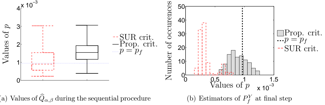
Figure 6: Distribution of the obtained values of \tilde{p}_j and \hat{Q}_{\alpha,\beta} obtained during the sequential procedure presented in Algorithms 1 and 2. Subfigure (a) compares for the SUR and the proposed criteria the distributions of all the values of \hat{Q}_{\alpha,\beta} obtained during the 10 repetitions of the sequential procedure. For a particular initial design of experiment, subfigure (b) compares the influence of the choice of the selection criterion on the distribution of 100 values of the estimators \tilde{p}_j of P_f^Y after having added n_{\text{add}} points.
