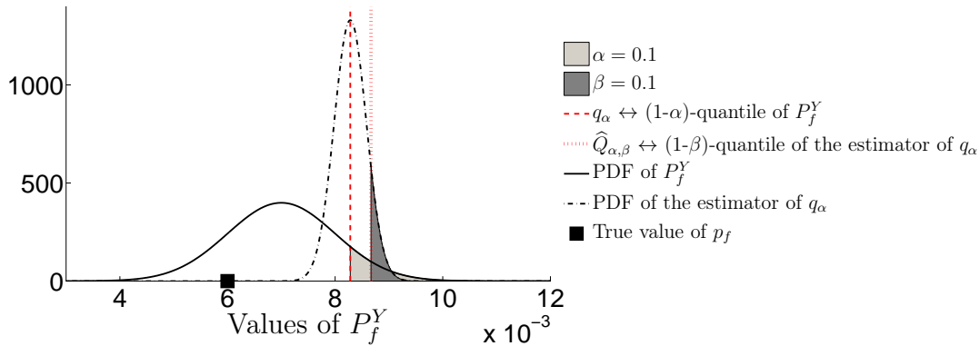
Figure 1: Graphical illustration of the meanings of \alpha , \beta , q_\alpha and \widehat{Q}_{\alpha,\beta} on a synthetic example.
