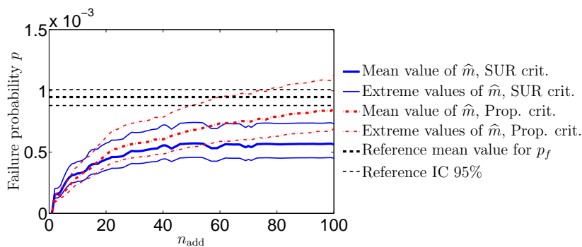
Figure 5: Convergence with respect to the number of added points n_{\text{add}} of the estimator \hat{m} depending on the chosen selection criterion. For the reference value estimated with a Monte Carlo approach, IC 95% stands for 95% confidence interval. For the two compared criteria, the mean and the extreme (minimal and maximum) values are associated with 10 repetitions of the whole sequential procedure.
