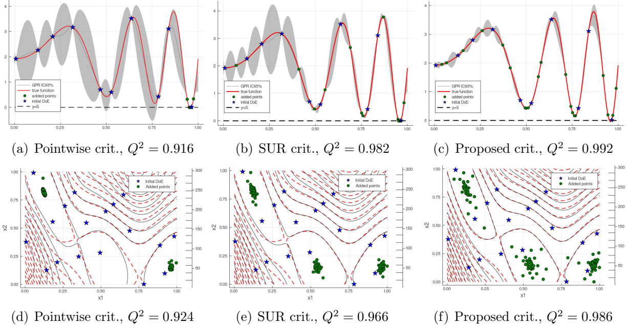
Figure 3: Comparison of the GPR-based surrogate models after adding n_{\text{add}} new code evaluations. In each subfigure, function y is represented in red (in solid line for the oscillating function and in dotted line for the Branin function), the blue stars indicate the positions of the \ell initial training points, and the green circles indicate the positions of the new code evaluations. For the oscillating function, the grey area corresponds to the 95% prediction interval provided by the surrogate model, when the contour lines associated with the conditioned mean are in black solid line for the Branin function. Here, Q^2 is the classical metric of learning performance on test data calculated as one minus the predictive residual error sum of squares (PRESS) divided by the total sum of squares (TSS).
