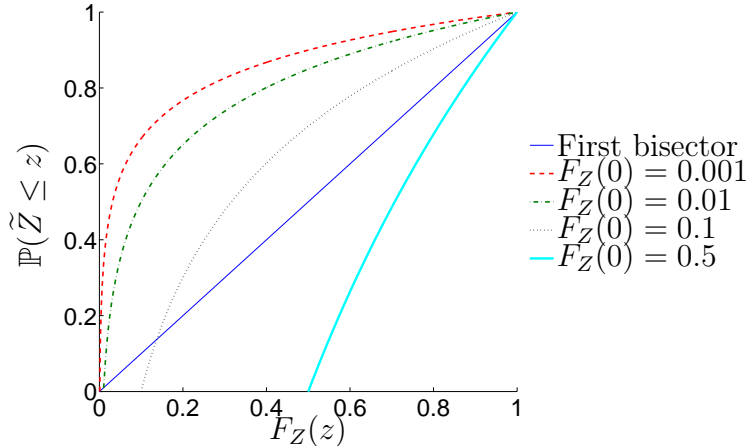
Figure 2: Concentration of the points generated by Algorithm 1 on the low values of y (with n_{\max} = +\infty ).
