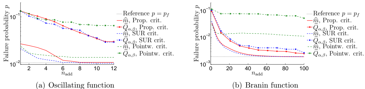
Figure 4: Convergence with respect to the number of added points n_{\text{add}} of the estimators \hat{m} and \hat{Q}_{\alpha,\beta} depending on the chosen selection criterion.
