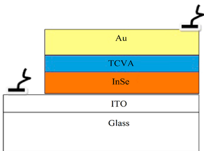
Fig. 5. Schematic layout of hybrid ITO/InSe/TCVA/Au solar cell. Adopted from Al Garni and Darwish (2017).
