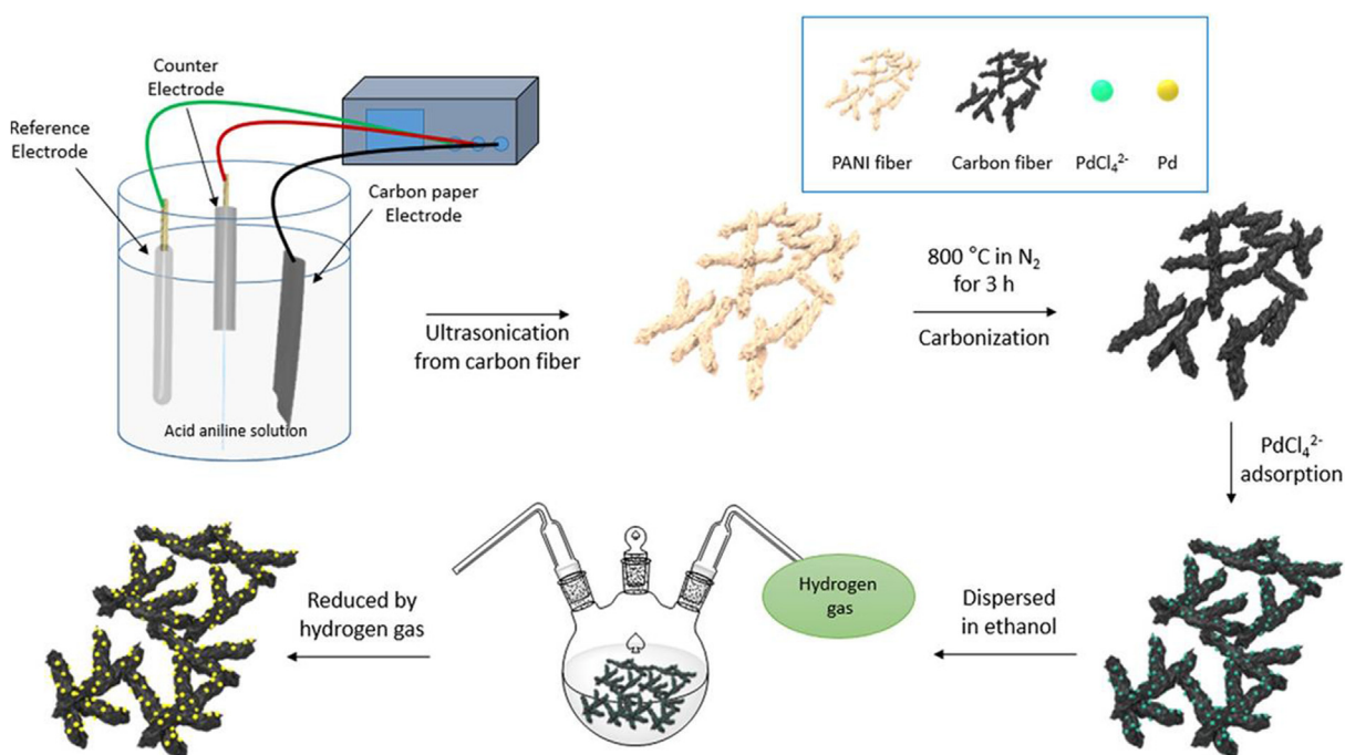
Fig. 6. Schematic diagram of synthesizing hybrid Pd/N-C material. Adopted from Shim et al. (2018).
