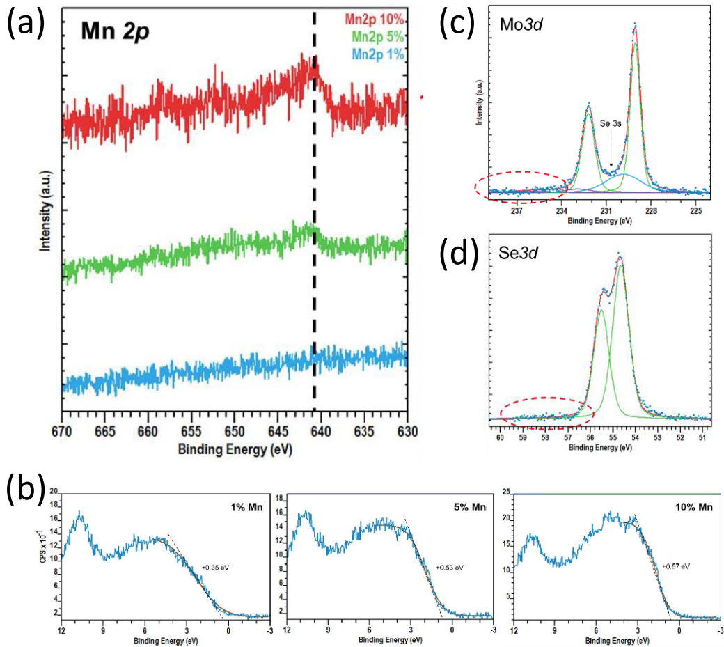
Figure 7. (a) Mn 2p core-level and (b) valence band spectra for \text{Mo}_{1-x}\text{Mn}_x\text{Se}_2 samples with x = 0.01 ; 0.05 and 0.1. (c) Mo 3d and (d) Se 3d core-level spectra for the sample containing 5% of Mn. Solid lines are fits.
