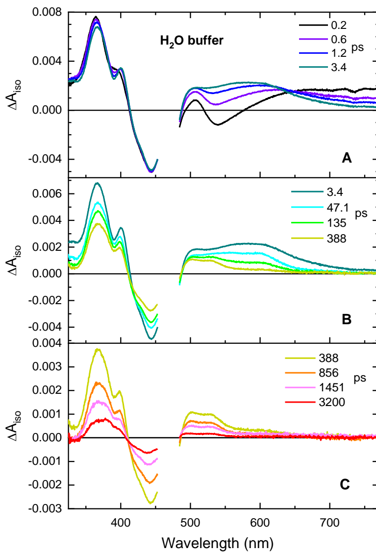
Figure 2. Isotropic transient absorption spectra of DsNewPHL in \text{H}_2\text{O} buffer, at selected pump-probe delays after fs excitation at 470 nm.
