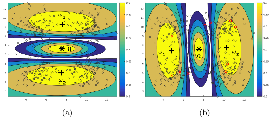
Figure 4: Contour surfaces of the credal partition obtained by (a) ECM and (b) SECM. Centroids for singletons and the universe are designed by crosses and stars. Label constraints are highlighted in red.
