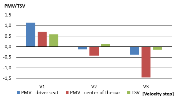
Fig. 14 Comparison between the PMV and TSV indexes
