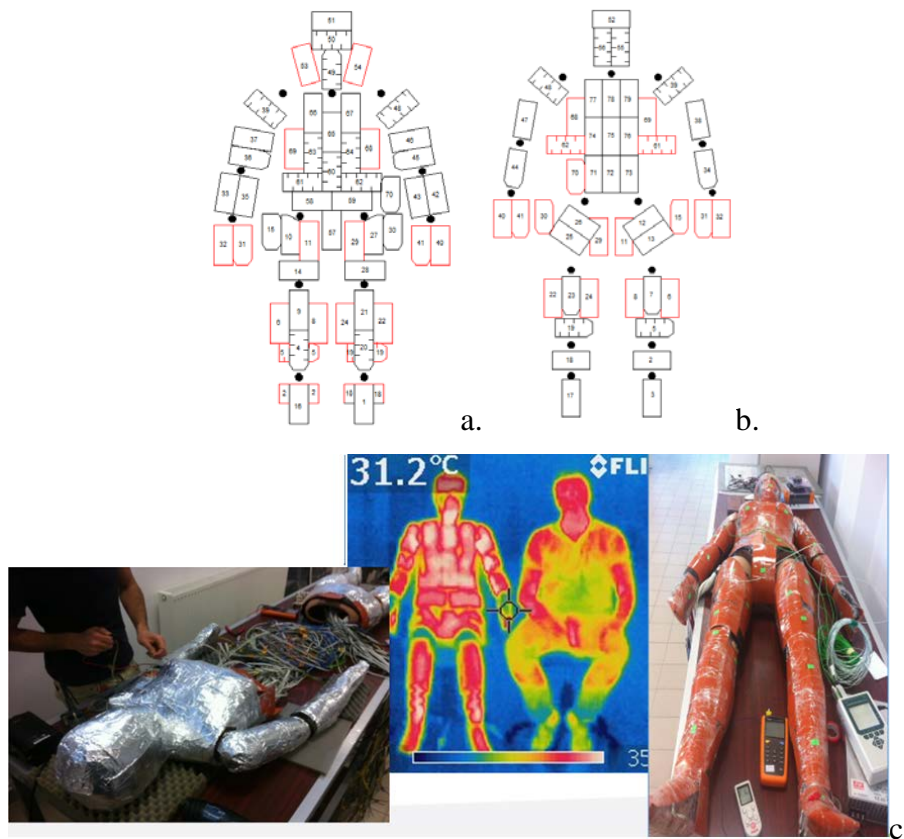
Fig. 4. Thermal manikin employed in this study: distribution of the heating elements on the individually anatomic zones controlled (red patches are corresponding to the other side of the manikin): a) front view, b) back view, c) general appearance and comparison with the anatomic distribution of skin temperature of a human
