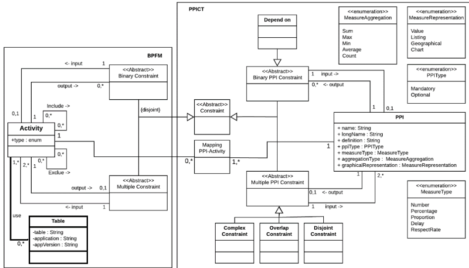
Fig. 6. PPIC Metamodel linked to BPFM Metamodel
