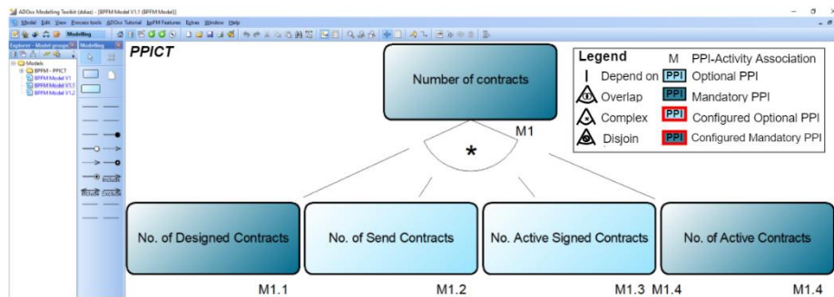
Fig. 3. PPICT (Numbers of Contracts PPIs Family model)
