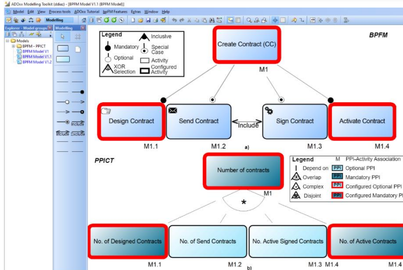
Fig. 5. a) BPFM Configuration, b) PPICT conforming configuration
