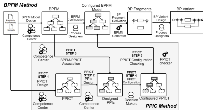
Fig. 2. PPIC Method's steps
