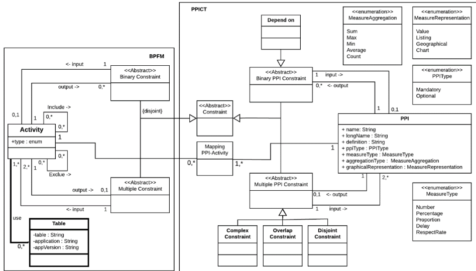
Fig. 6. PPICT Metamodel linked to BPFM Metamodel
