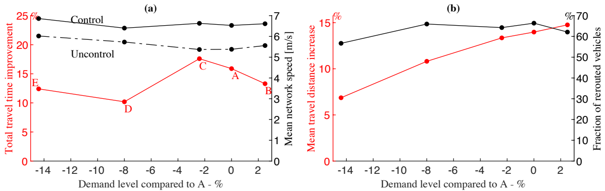
Fig. 12: Influence of the initial network loading (Manhattan network). (a) total travel time improvement ( V_{III} ); (b) mean travel distance increases for rerouted vehicles ( D_{up} ) and fraction of rerouted vehicles ( F_r ).
