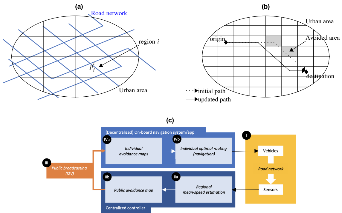
Fig. 1: The control concept (a) public avoidance maps; (b) individual avoidance map and impacts of the vehicle trajectory; (c) overall sketch.
