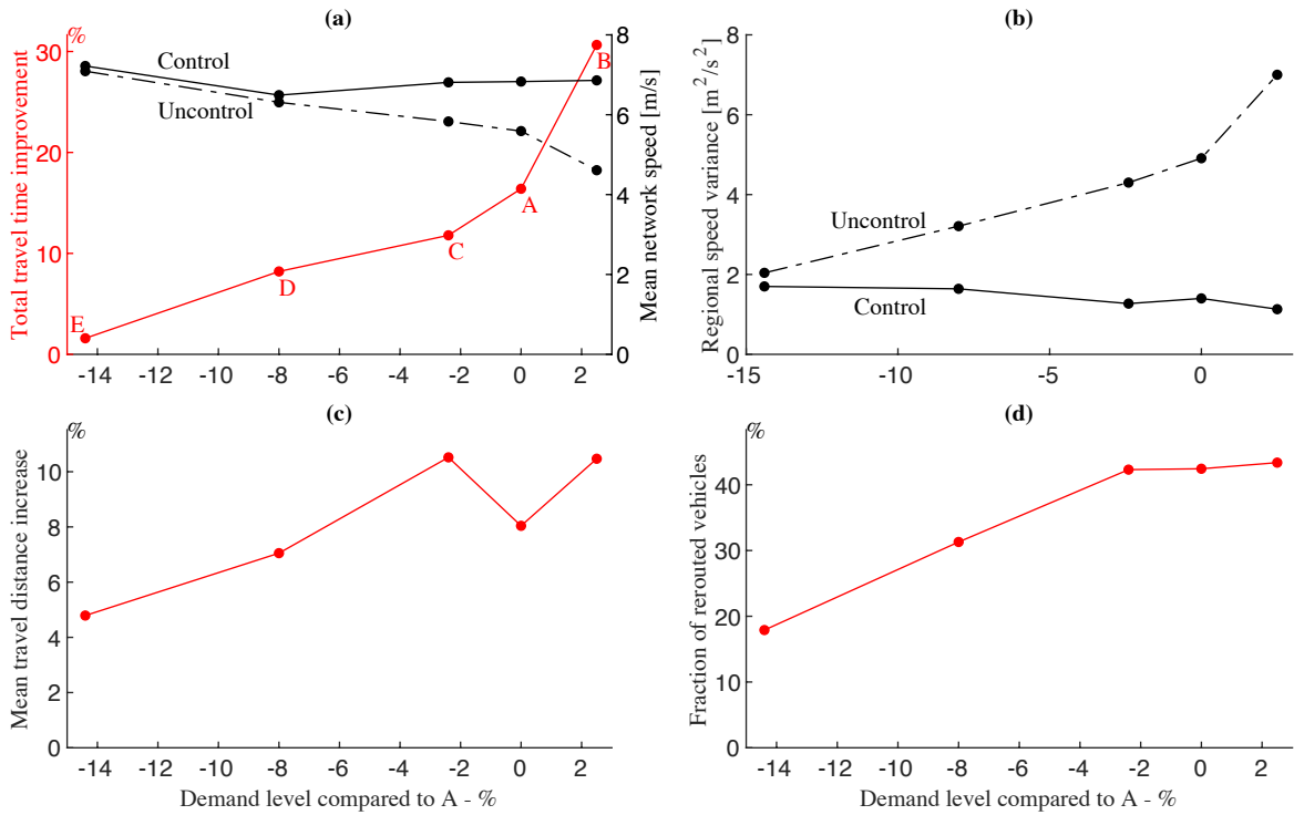
Fig. 8: Influence of the demand level on the controller performances (Manhattan network). (a) total travel time improvement ( V_{tt} ); (b) network speed homogeneity; (c) mean travel distance increases for rerouted vehicles ( D_{up} ); (d) fraction of rerouted vehicles ( F_r ).
