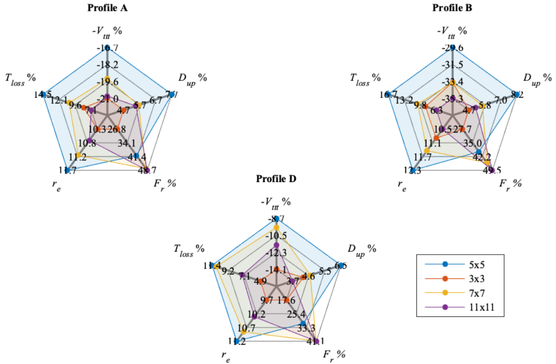
Fig. 10: Influence of the region sizes for different demand profiles (Manhattan network); V_{ttt} : total travel time reduction; D_{up} : mean individual travel distance increase; F_r : Fraction of rerouted vehicles; r_e : mean number of route events; T_{loss} : mean individual travel time loss.
