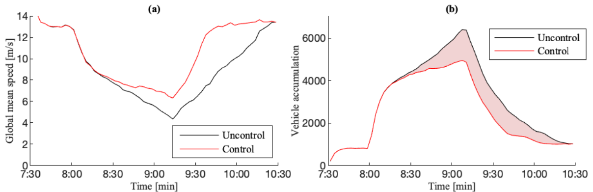
Fig. 13: Evolution of (a) the global mean speed and (b) the vehicle accumulation for the reference scenario (Lyon63V network).
