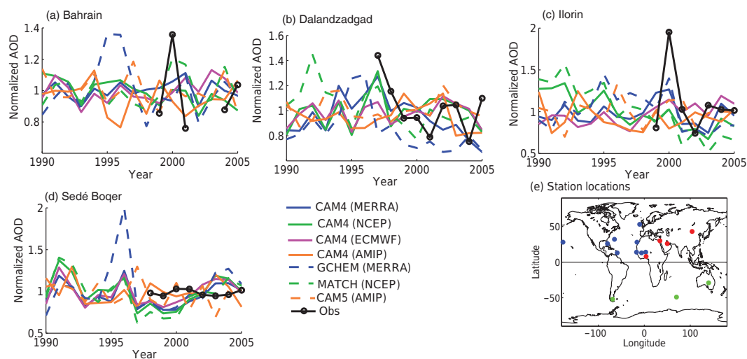
Figure 2. Time series of annual average AOD for model simulations (based on dust only), compared with AERONET observations in Table 2 for: (a) Bahrain, (b) Dalandzadgad, (c) Ilorin and (d) Sedé Boqer for each of the different model versions (colors are the same as in Fig. 1). Observational data from AERONET stations (citations listed in Table 2). The annual means are divided by the long-term mean to allow comparison with seasonal variability, since they are similarly normalized (Fig. S8). A map (e) with station locations for concentration (blue; Fig. 1), AOD (red; Fig. 2) and Southern Hemisphere analysis (green; Fig. 5).
