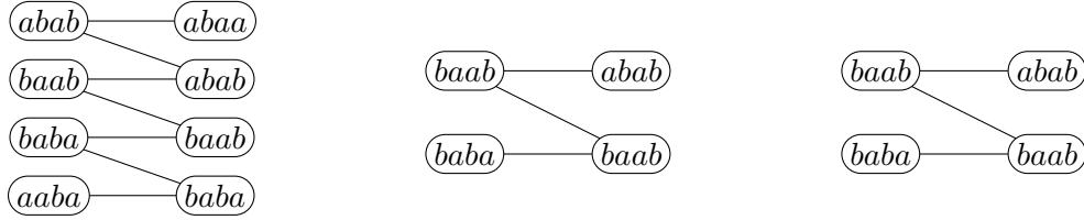
Figure 3: The graphs of \mathcal{E}_{4,4}(a) (on the left), \mathcal{E}_{4,4}(abaaba) (on the center) and H (on the right).
