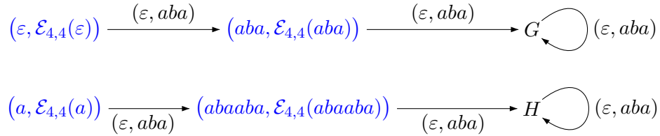
Figure 4: Graph of graphs of the Fibonacci set S .
