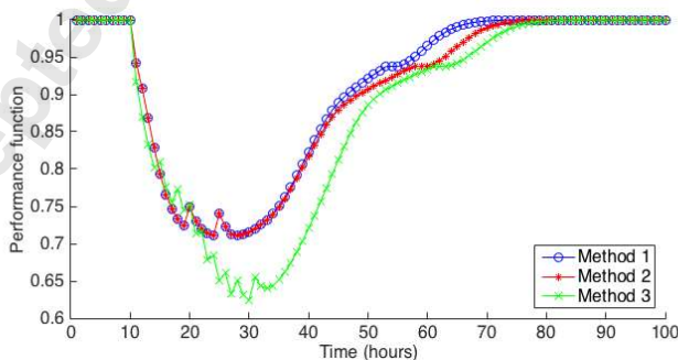
Fig. 6. The evolution of system performance with three methods, dv=10
