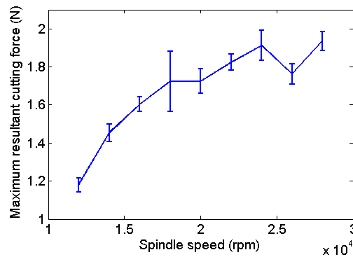
Figure 8 – Cutting force evolution when increasing cutting speed.
