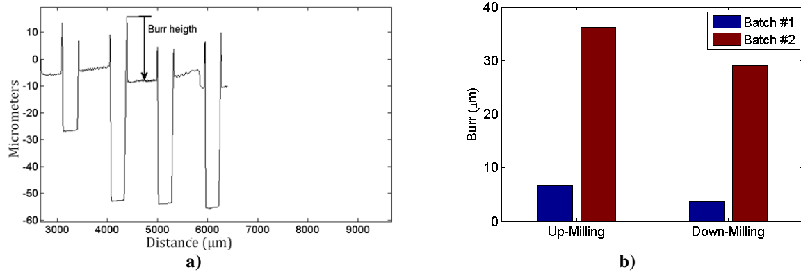
Figure 3 – Analysis of burr formation: a) Measurement of top burr height; b) Comparison between burr height for batch #1 (feed of 2.5 µm/tooth and depth of cut of 50 µm) and batch #2 (feed of 2.5 µm/tooth and depth of cut of 40 µm).
