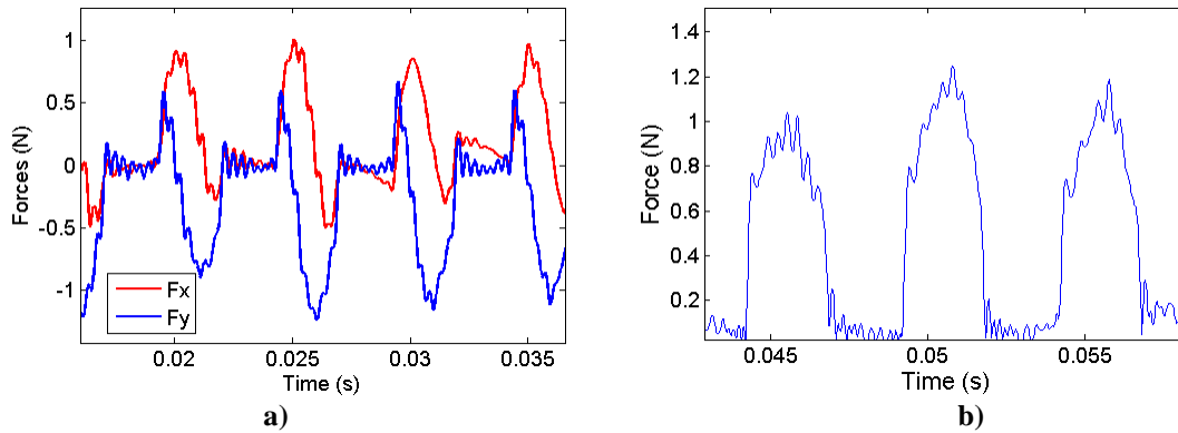
Figure 7 – Cutting force measurement for slot #1: a) Cutting force on direction X and Y; b) Resultant cutting force.
