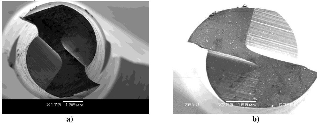
Figure 1 – SEM images of the microtools. a) Performance Micro Tool; b) Mitsubishi Materials.
