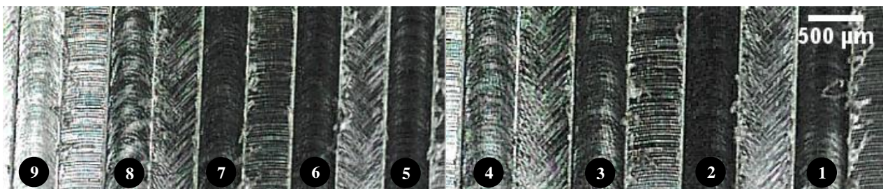
Figure 4 – Machined slots image taken with a Handheld Digital Microscope (slots width: 500 µm).
