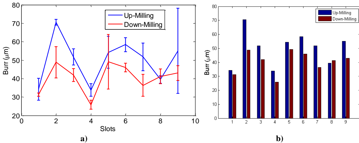
Figure 6 – Top burr height measurements for slots 1-9: a) Graph with error bar representation using the standard deviation; b) Bar graph for a better visualization of the results.
