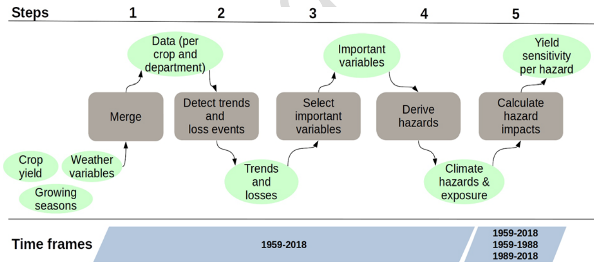
83 Figure 1: Workflow of the analysis in five steps. Ellipses are inputs and outputs, rounded rectangles denote operations 84 and parallelograms the time frames for which analyses were carried out.
