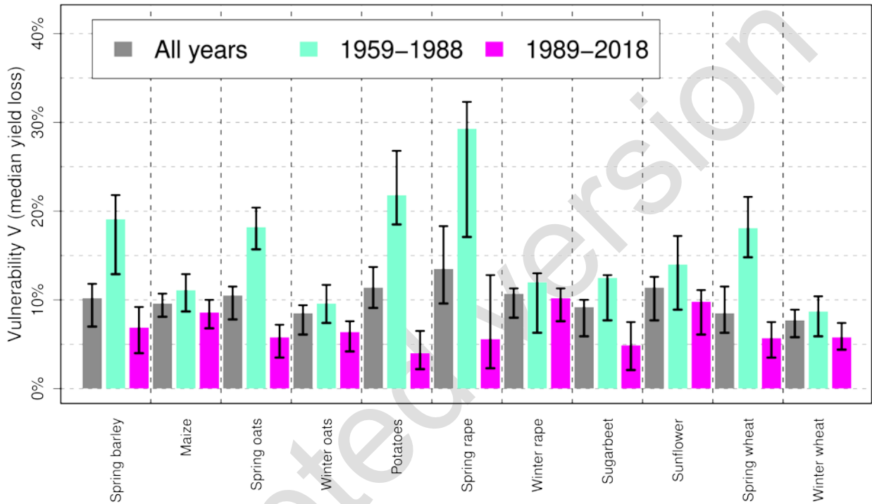
438 439 Figure 7: Vulnerability (exposure-weighted yield loss in % of expected yield, V from eq. 7) of weather hazards on crop 440 production in an average year for three time frames: 1959-2018, 1959-1988 and 1989-2018. Black lines denote the 5% 441 and 95% percentile range of 500 bootstrapped estimates.
