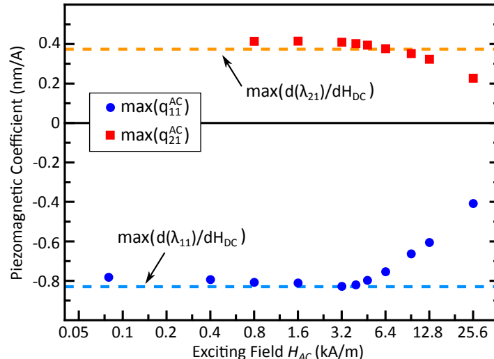
Fig. 3. Longitudinal (circles) and transverse (squares) piezomagnetic coefficient measured for NiFe 2 O 4 as function of the exciting field H_{AC} at 80 Hz (semi-log 2 plot) and at the optimum bias field H_{DC} . The strain derivatives are plotted in dotted line for comparison.
