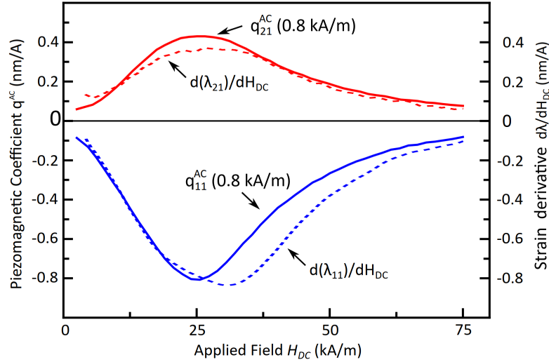
Fig. 2. Strain derivatives (dotted line) of NiFe 2 O 4 for longitudinal d(\lambda_{11})/dH_{DC} and transverse d(\lambda_{21})/dH_{DC} direction. Longitudinal ( q_{11}^{AC} ) and transverse ( q_{21}^{AC} ) piezomagnetic coefficient (continuous line) measured with an exciting field H_{AC} = 0.8 kA/m at 80 Hz as function of the bias field H_{DC} .
